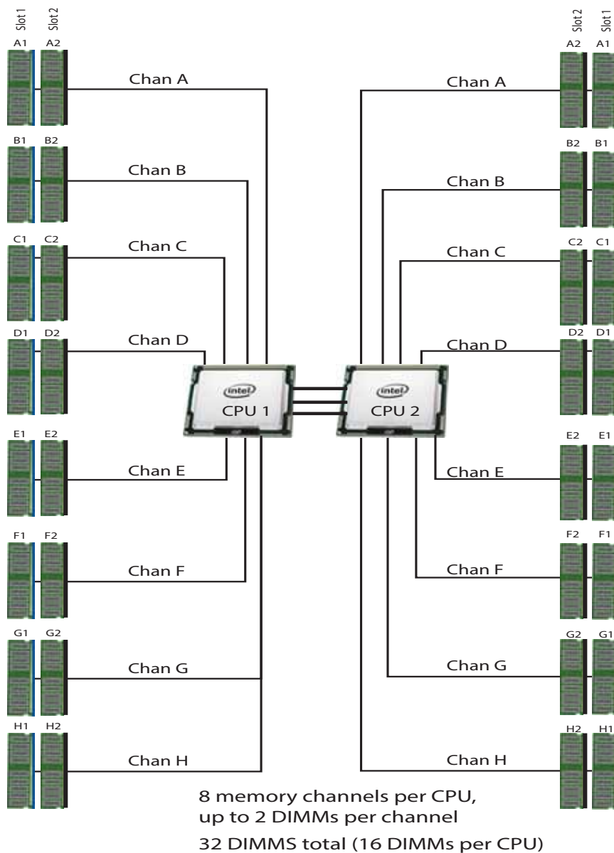
Figure 6 Cisco Compute Hyperconverged HClAF220C M7 All-NVMe/All-Flash Servers Memory Organization
