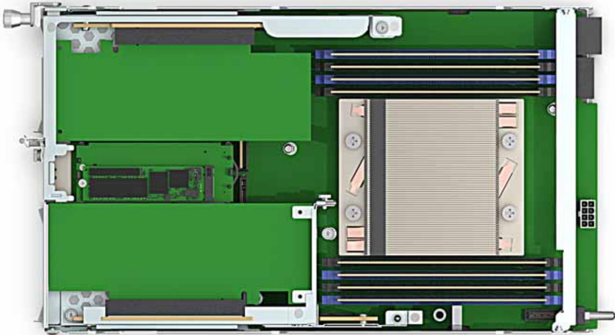
Figure 5 Cisco Compute Hyperconverged with Nutanix XE130c M8 Edge Server System Board
