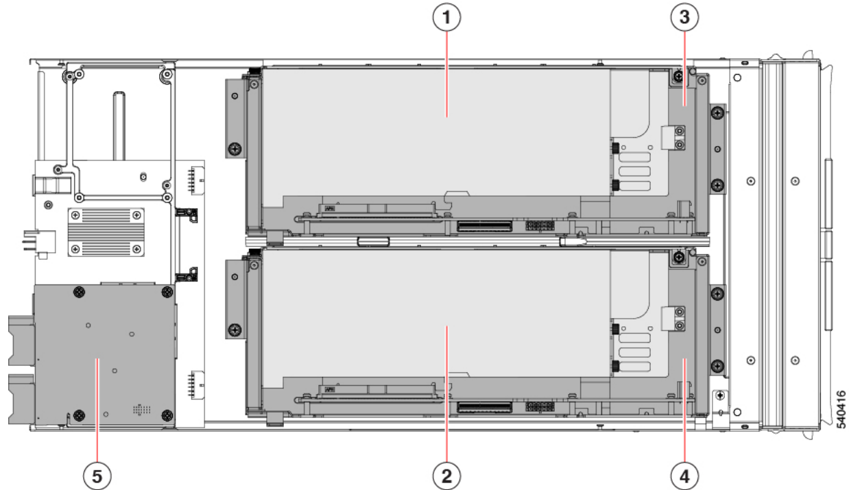
Figure 3 A Top View Of The Cisco Compute Hyperconverged X580p PCIe Node System Board
