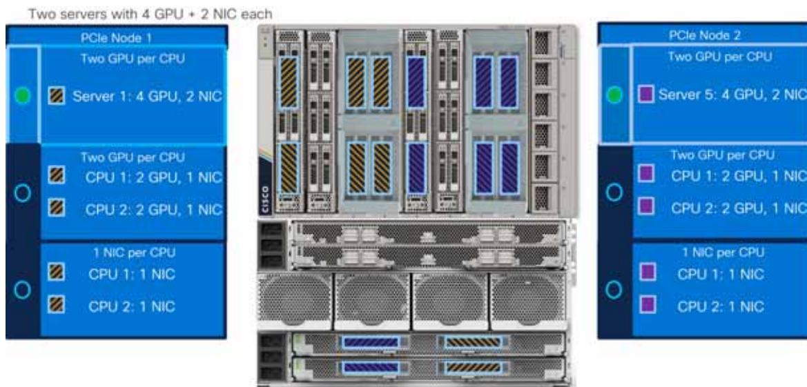
Figure 4 Two servers with 4x GPU + 2 NIC each
