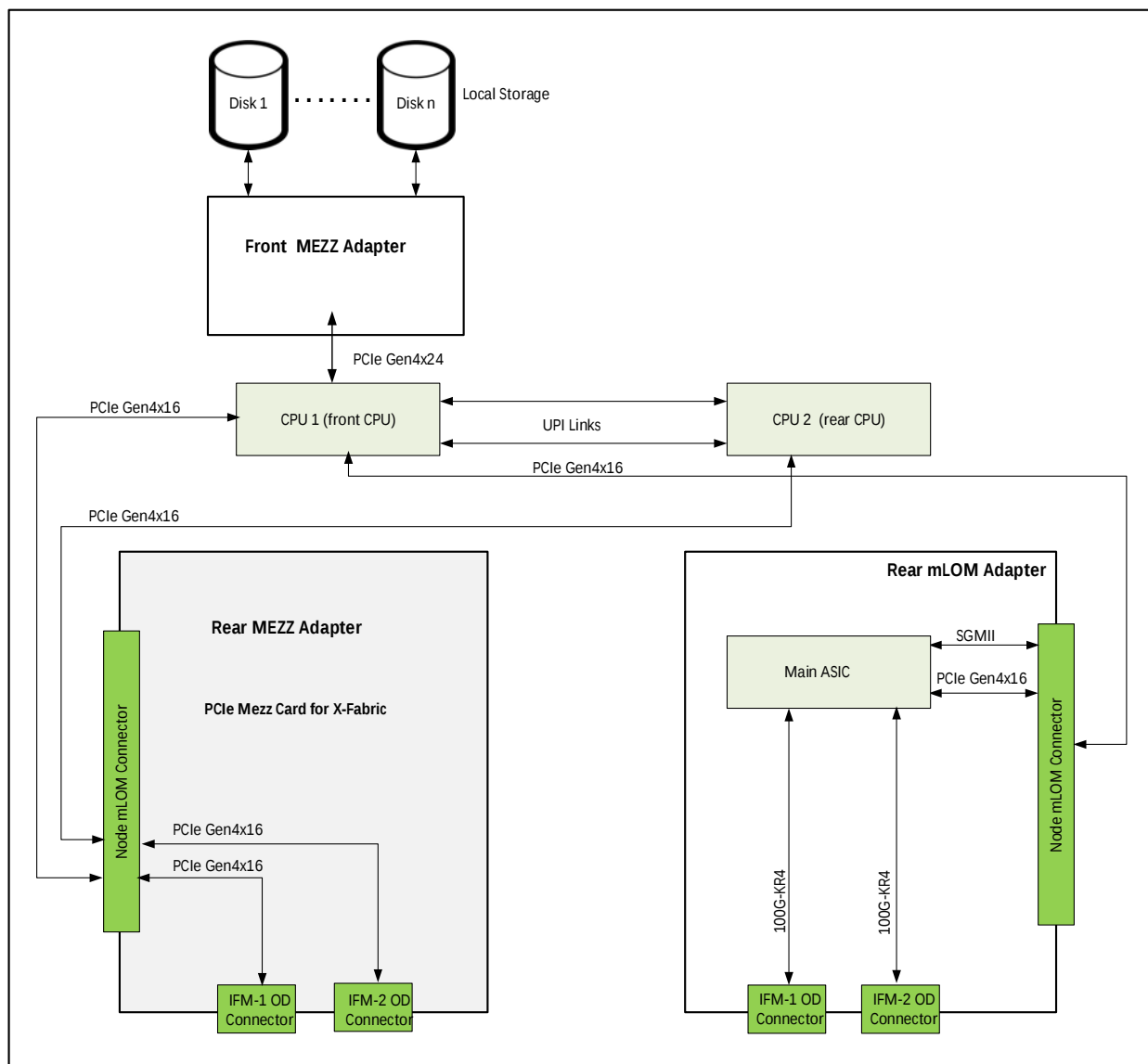
Figure 8 Compute Node Simplified Block Diagram (VIC 100G with Drives)
