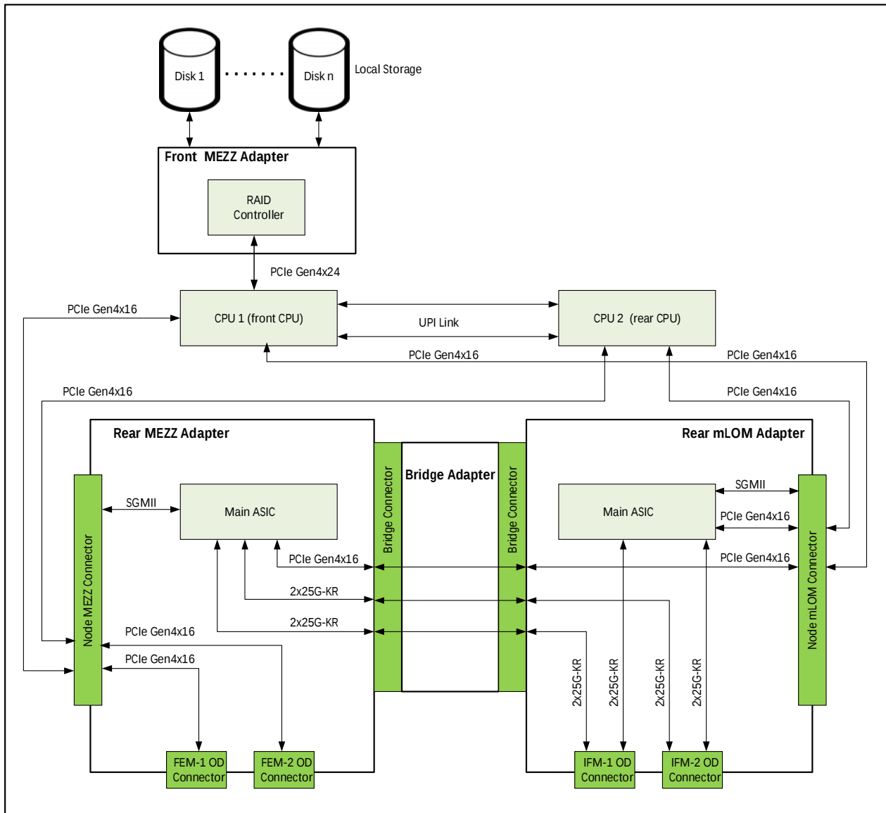
Figure 7 Compute Node Simplified Block Diagram (VIC 25G with Drives)
