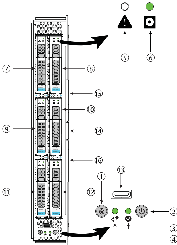
Figure 2 Cisco Compute Hyperconverged HCIXNX215c M8 All-NVMe Compute Node Front View (Drives option)
