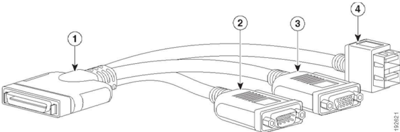
Figure 6 KVM Cable
