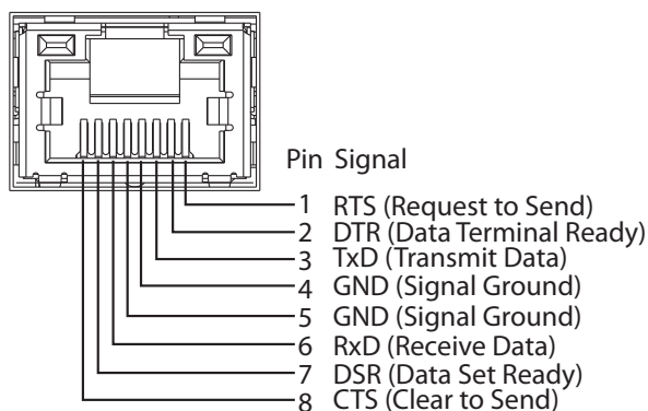
Figure 5 Serial Port (Female RJ-45 Connector) Pinout
