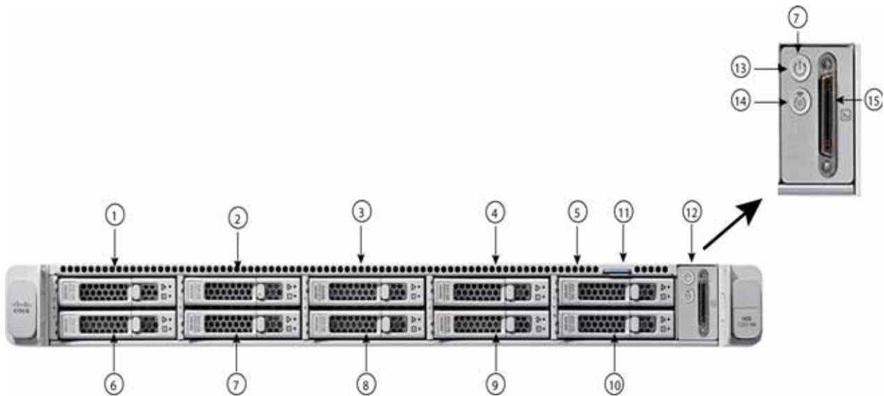
Figure 2 Detailed Chassis Front View
