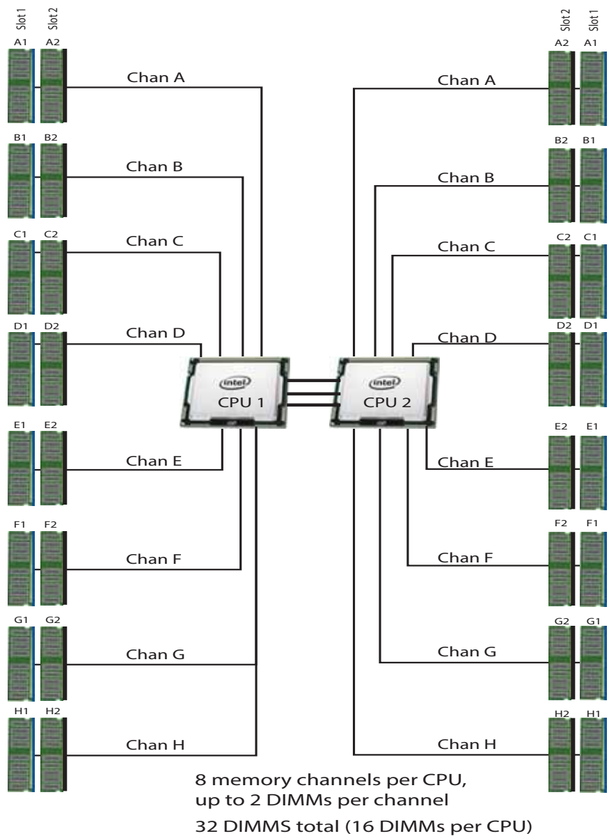
Figure 4 Memory Organization
