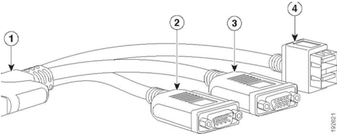
Figure 7 KVM Cabbble
