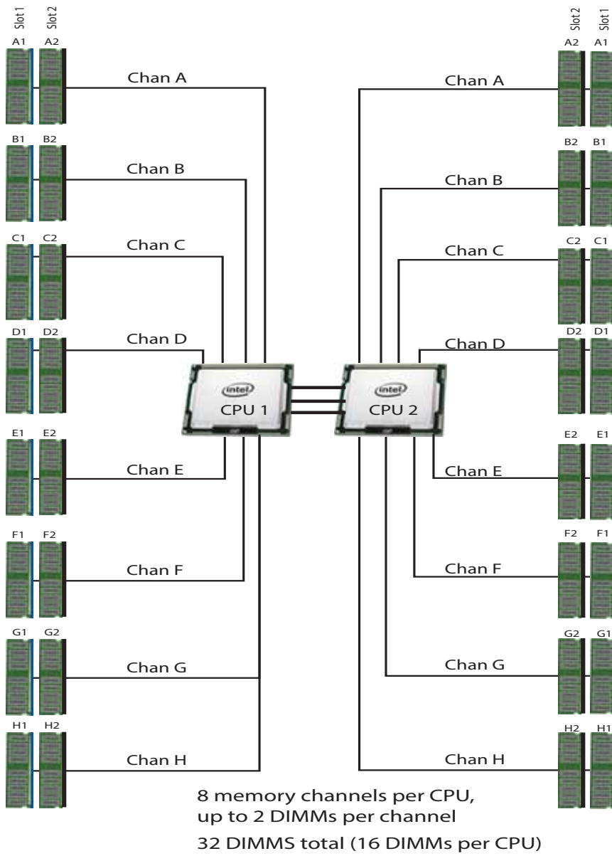
Figure 5 Memory Organization
