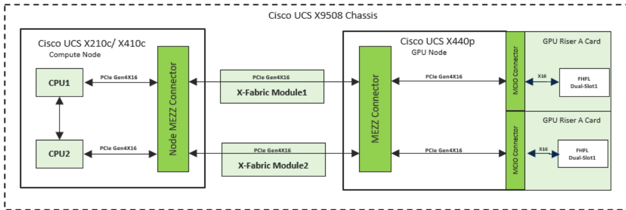
Figure 3 Cisco Compute Hyperconverged 440p PCIe Node Simplified Block Diagram with Riser A
