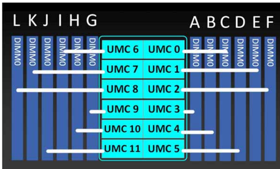
Figure 5 12-Channel Memory Organization
