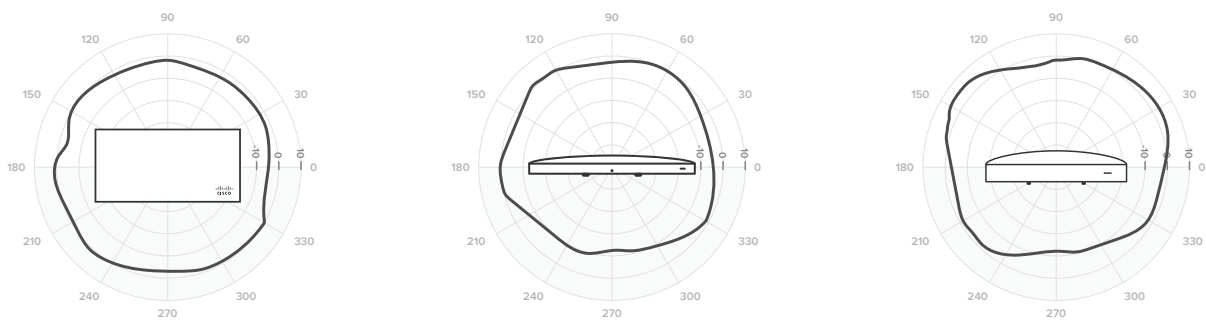
Radiation Pattern for 2.4GHz Antennas
