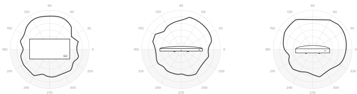
Radiation Pattern for 5GHz Antennas
