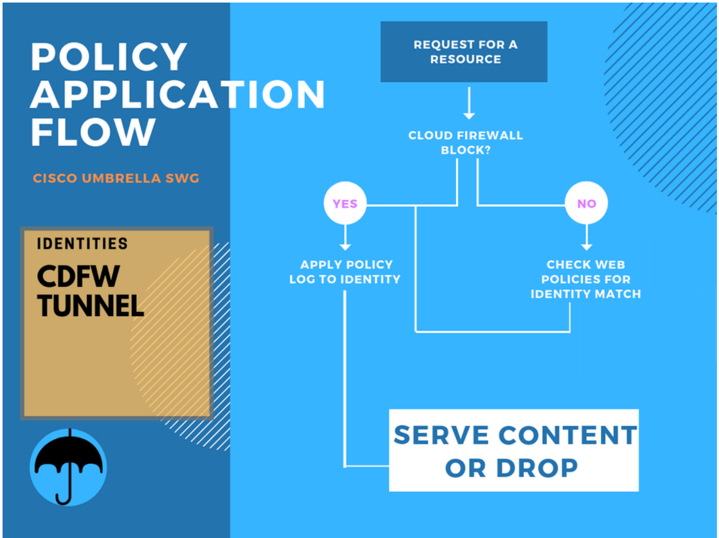
FlowChart-cdfw.png
