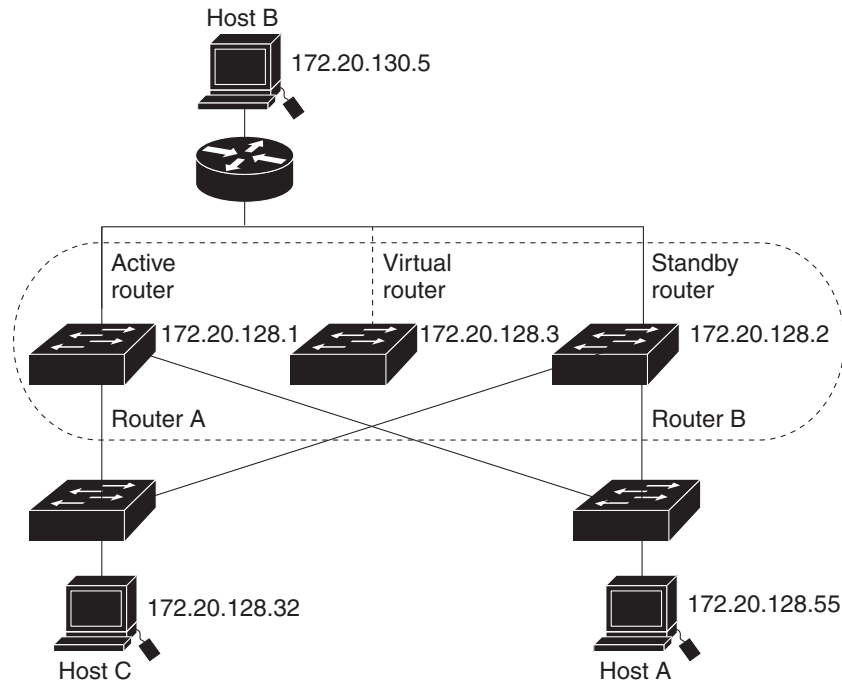
Figure 49-1 Typical HSRP Configuration
