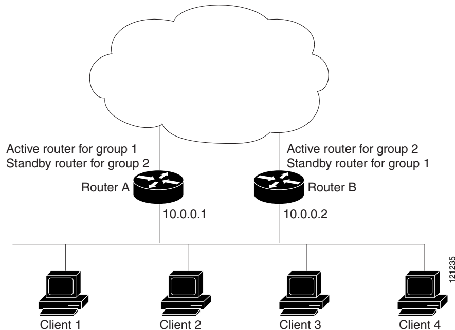
Figure 49-2 MHSRP Load Sharing
