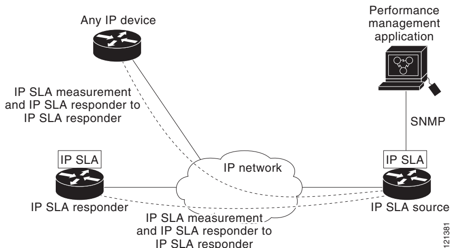
Figure 13 Cisco IOS IP SLAs Operation
