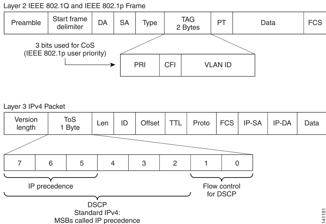
Figure 78 QoS Classification Layers in Frames and Packets
