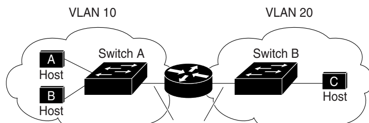
Figure 83 Routing Topology Example
