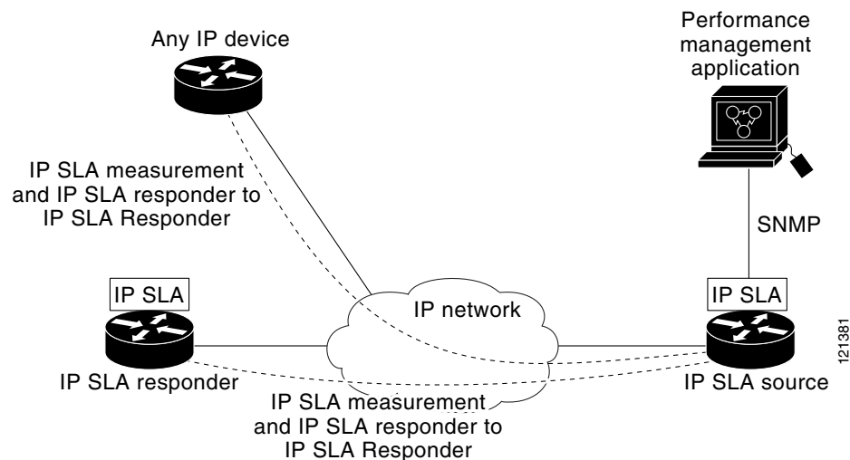
Figure 35-1 Cisco IOS IP SLAs Operation
