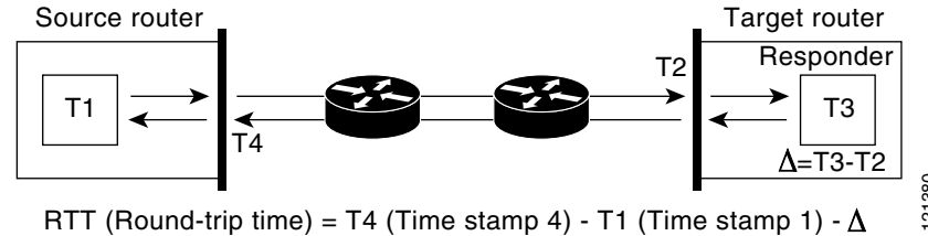
Figure 35-2 Cisco IOS IP SLAs Responder Time Stamping
