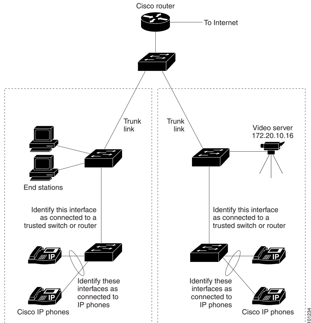
Figure 39-10 Auto-QoS Configuration Example Network
