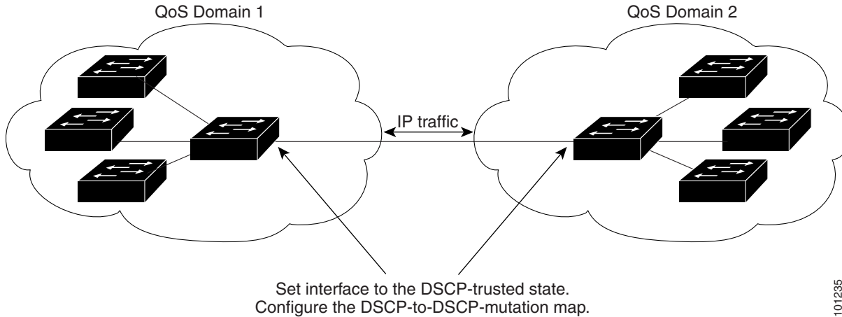
Figure 39-12 DSCP-Trusted State on a Port Bordering Another QoS Domain
