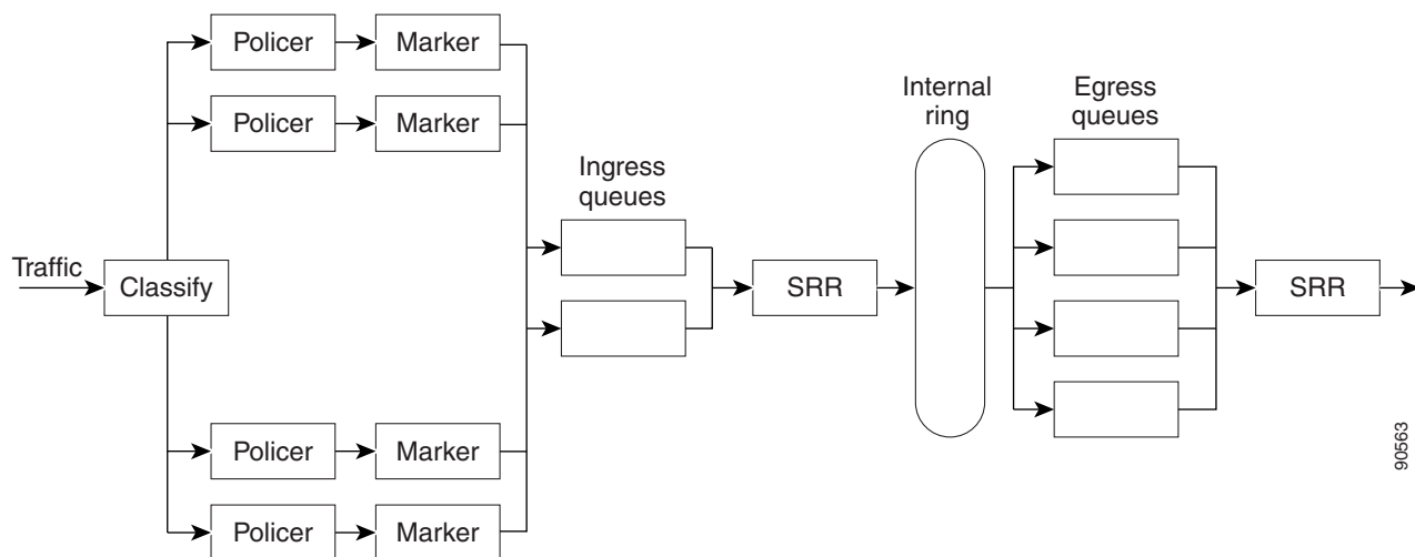
Figure 36-5 Ingress and Egress Queue Location
