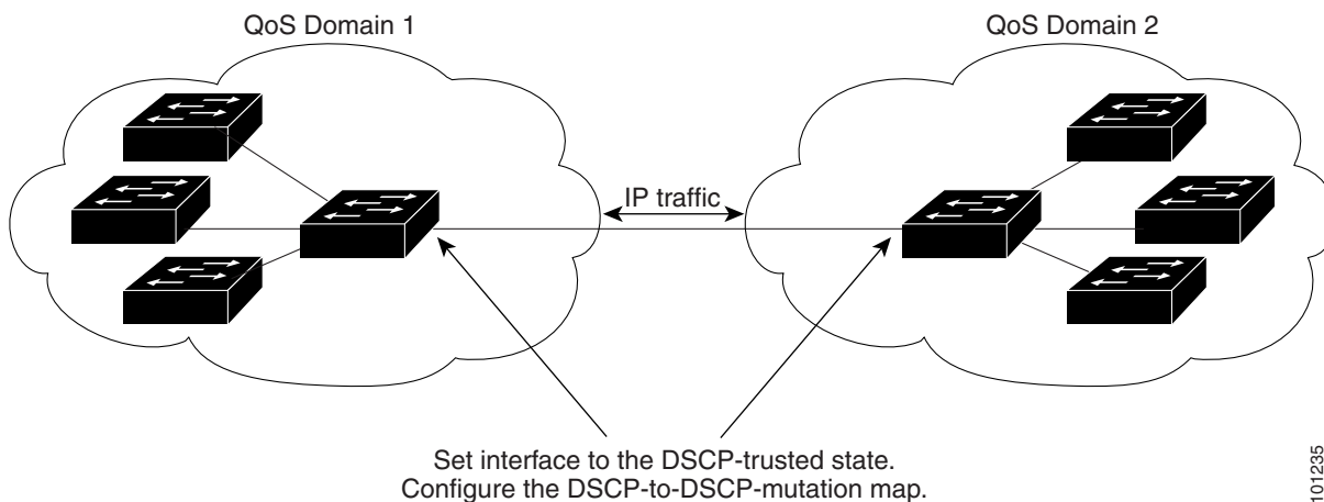
Figure 36-12 DSCP-Trusted State on a Port Bordering Another QoS Domain
