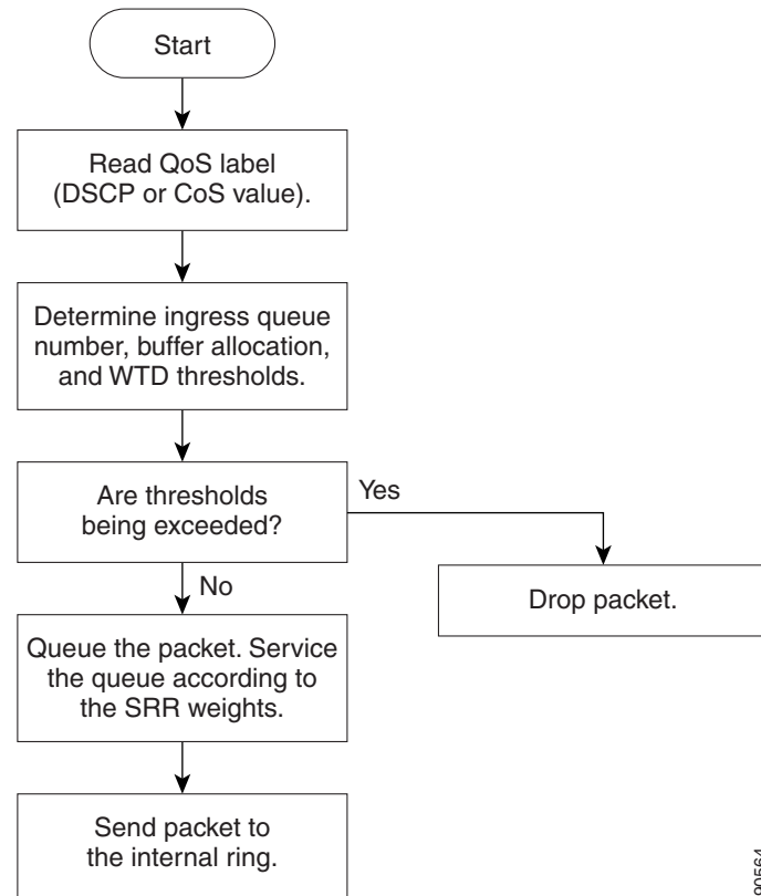
Figure 36-7 Queueing and Scheduling Flowchart for Ingress Ports
