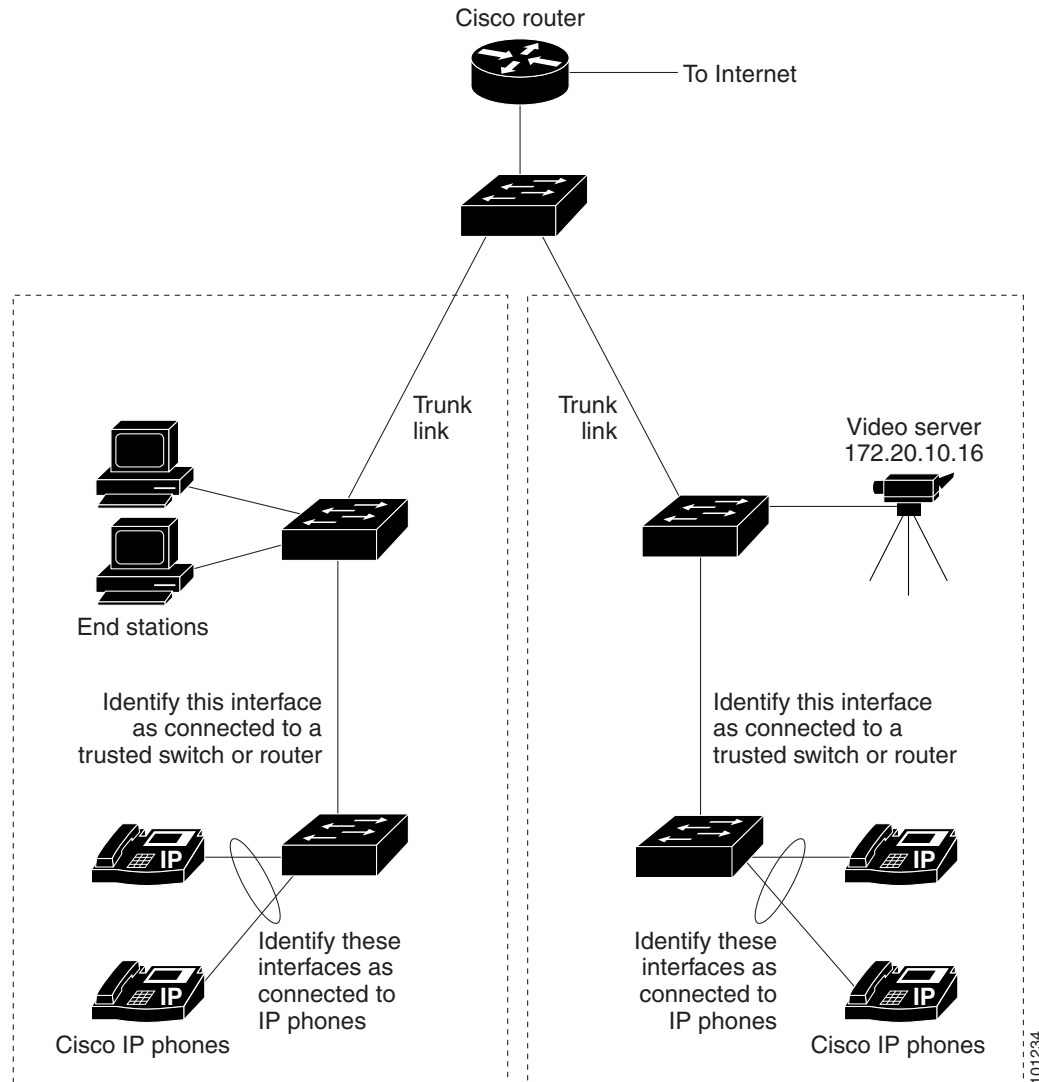
Figure 36-10 Auto-QoS Configuration Example Network
