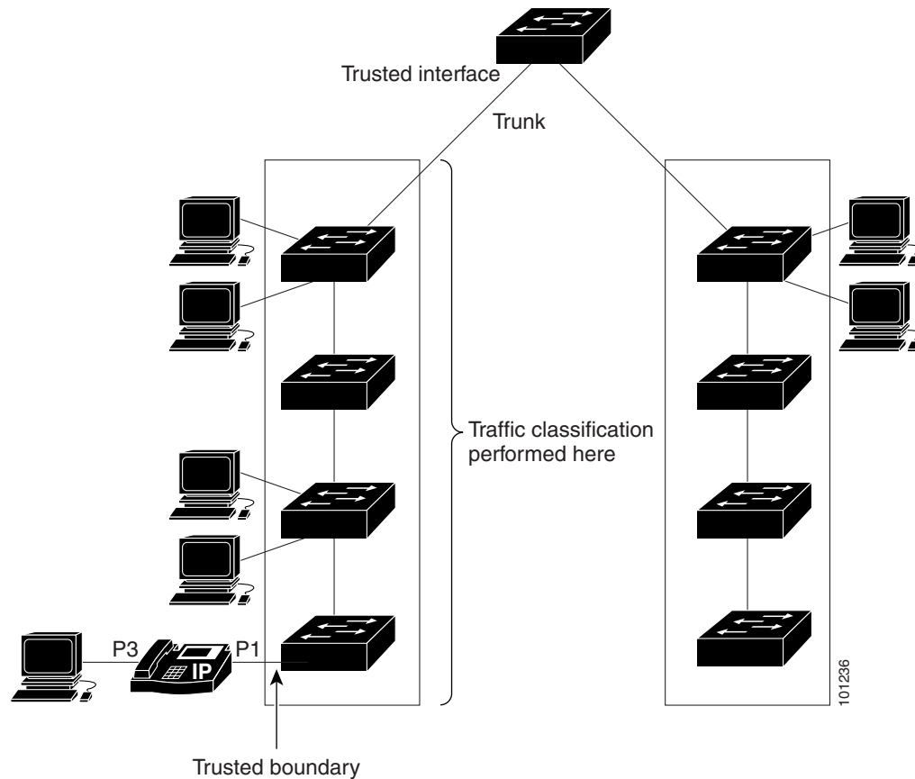
Figure 36-11 Port Trusted States within the QoS Domain
