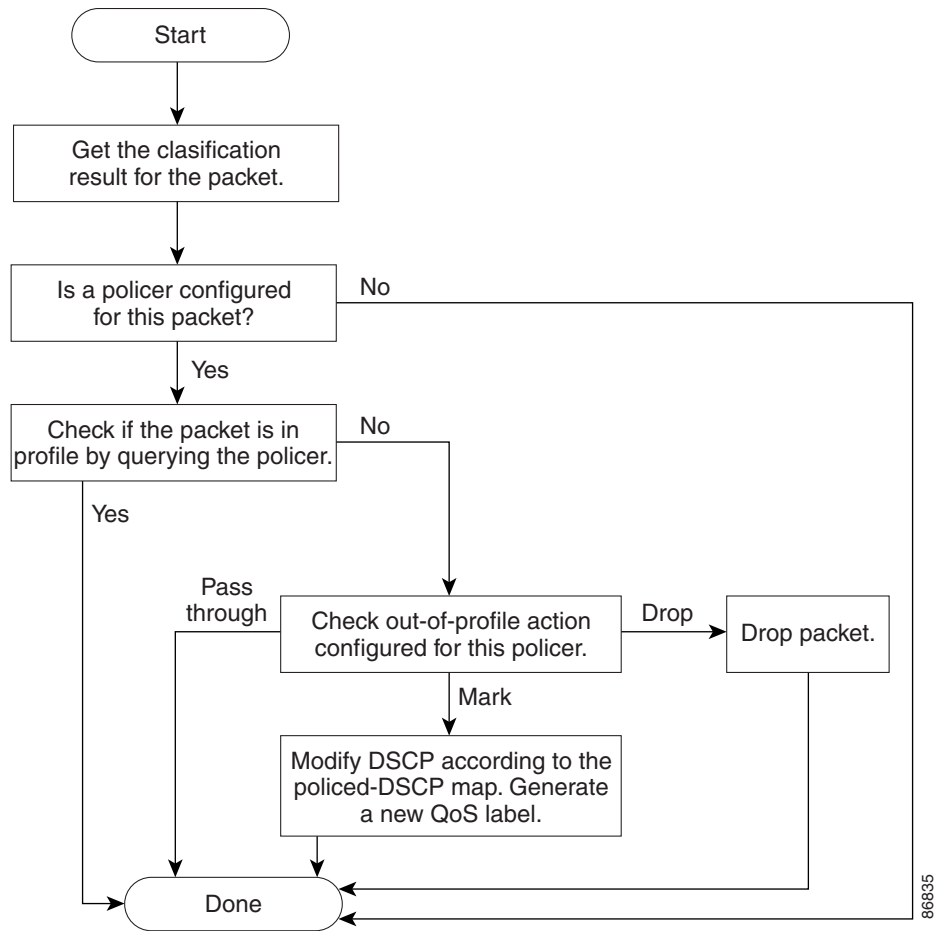
Figure 36-4 Policing and Marking Flowchart on Physical Ports
