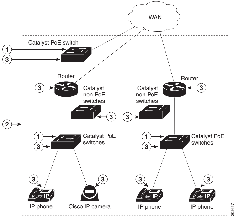
Figure 5-3 Multiple PoE Switches Example
