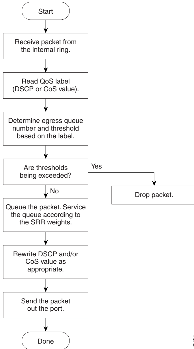
Figure 36-8 Queueing and Scheduling Flowchart for Egress Ports
