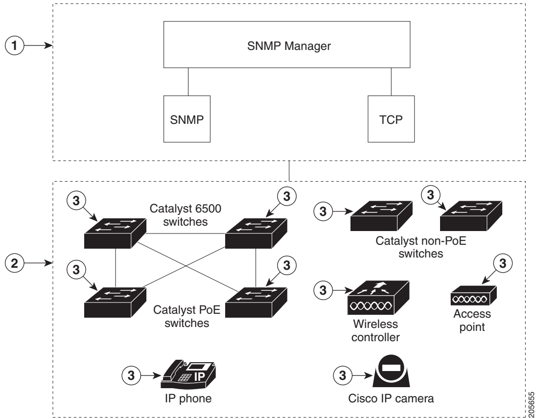
Figure 5-1 Typical Network
