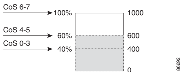
Figure 36-6 WTD and Queue Operation
