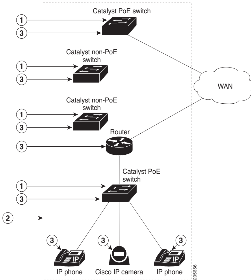
Figure 5-2 Single PoE Switch Example
