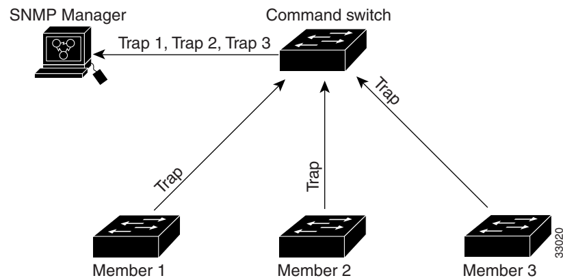
Figure 7-7 SNMP Management for a Cluster
