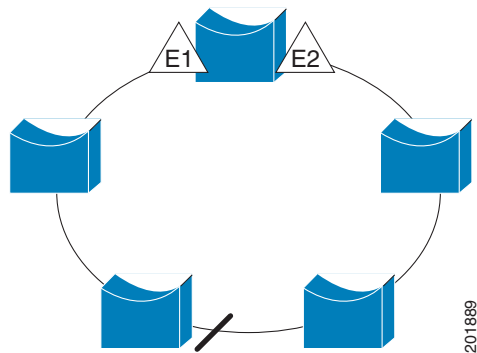
Figure 21-2 REP Ring Segment
