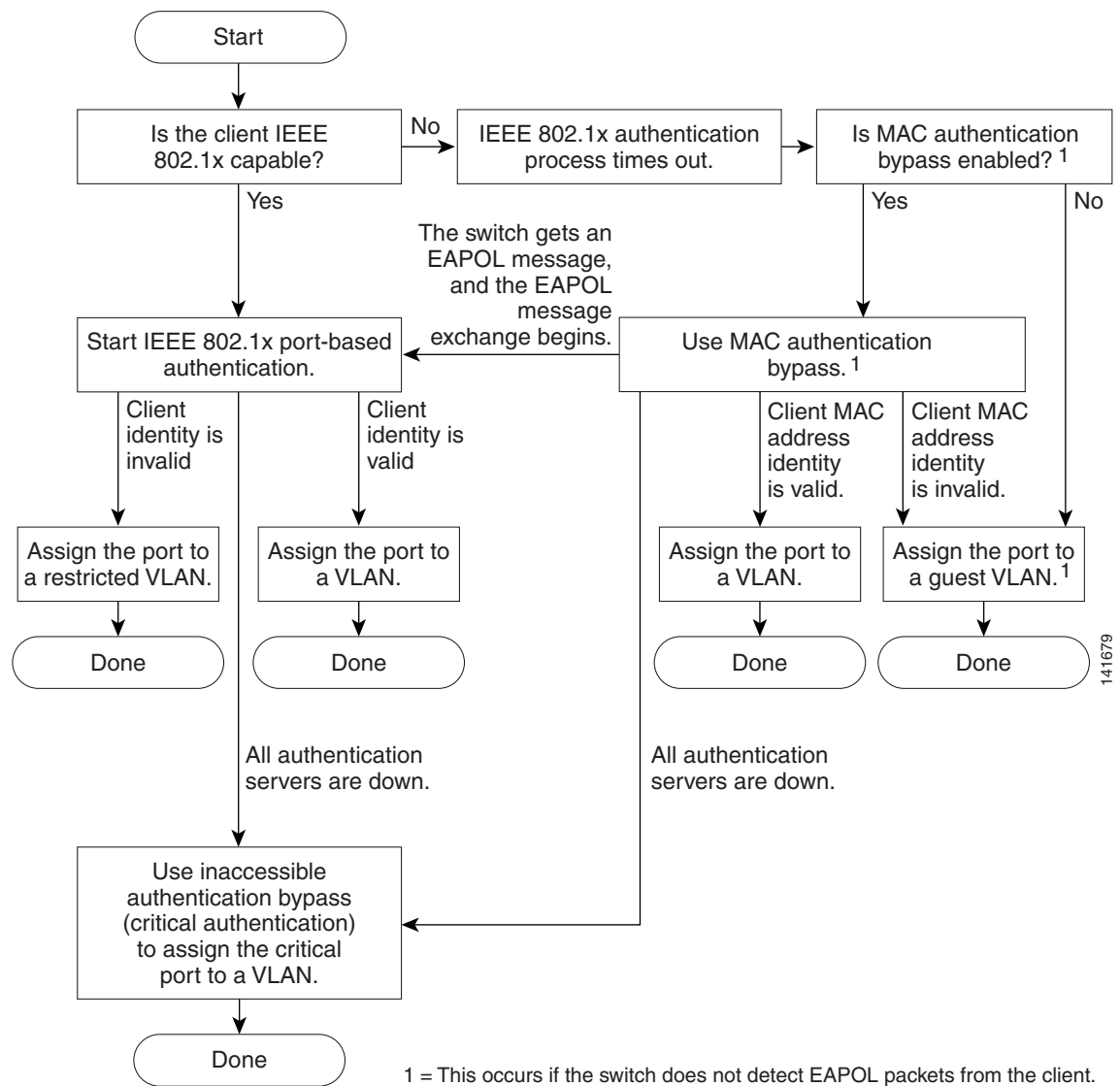
Figure 12-2 Authentication Flowchart
