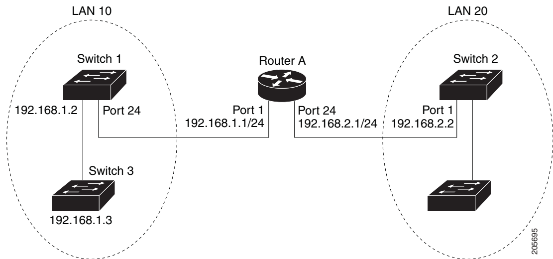
Figure 5-5 EnergyWise with IP Routing
