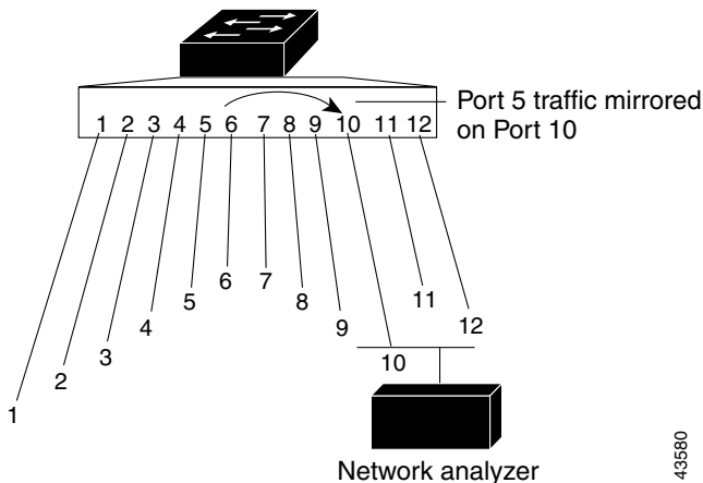
Figure 31-1 Example of Local SPAN Configuration on a Single Switch
