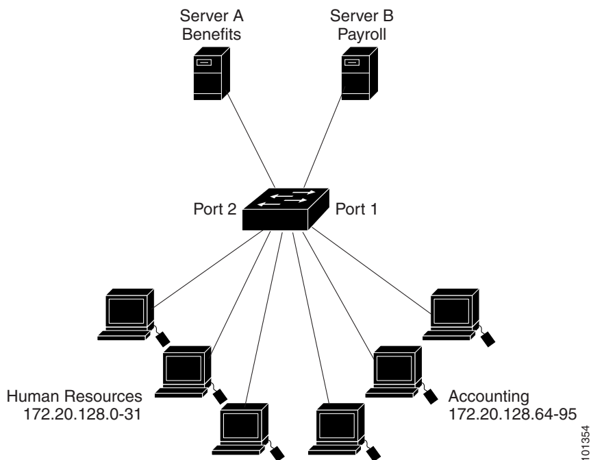
Figure 38-2 Using Router ACLs to Control Traffic
