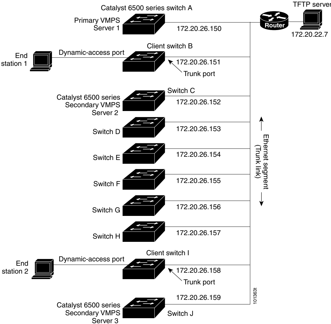
Figure 18-4 Dynamic Port VLAN Membership Configuration
