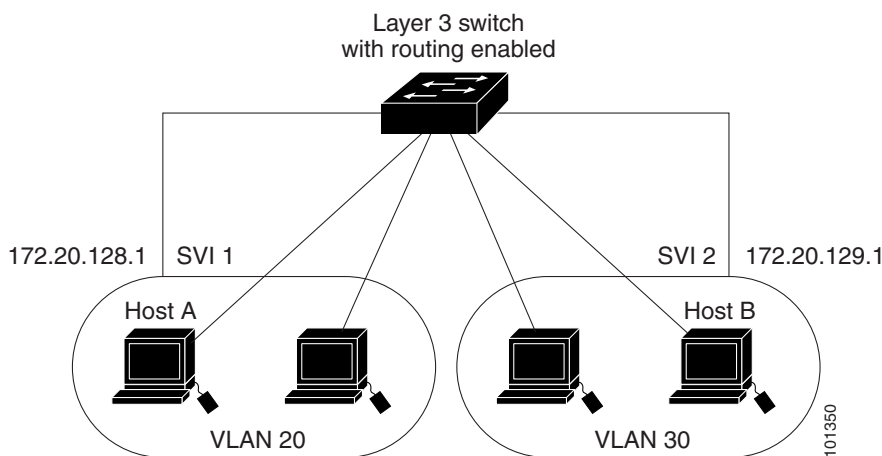
Figure 16-1 Connecting VLANs with a Layer 3 Switch
