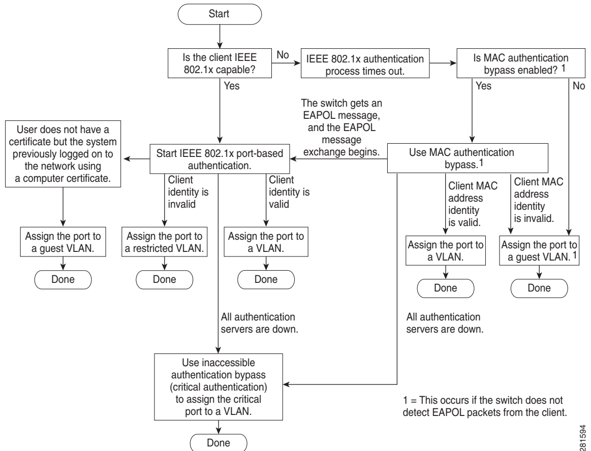
Figure 13-2 Authentication Flowchart
