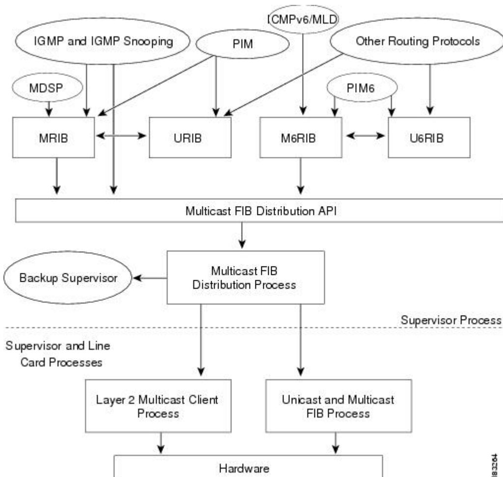
Figure 8: Cisco NX-OS Multicast Software Architecture
