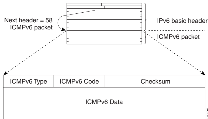
Figure 3-11 IPv6 ICMP Packet Header Format
