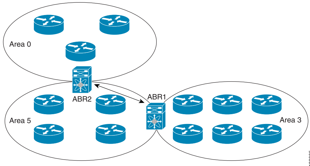
Figure 7-4 Virtual Links
