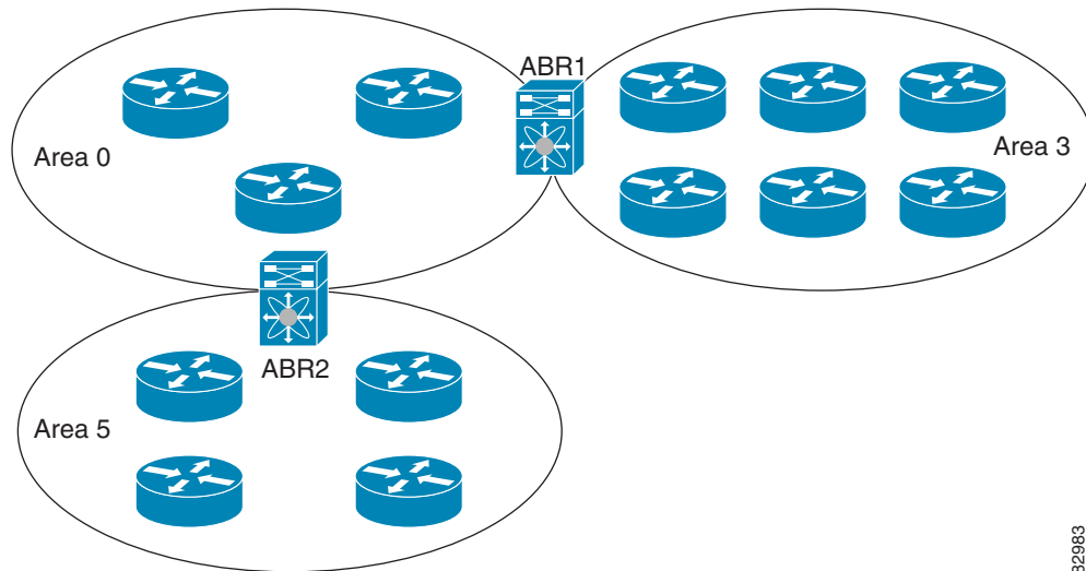
Figure 6-2 OSPFv2 Areas
