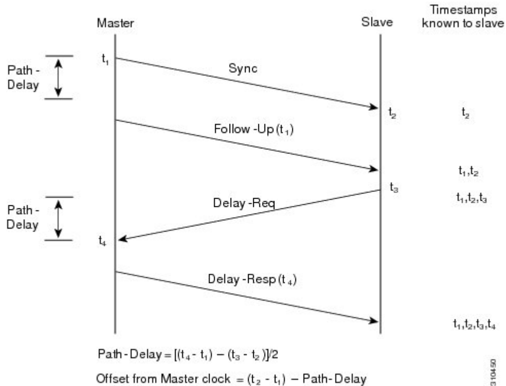
Figure 2: PTP Process
