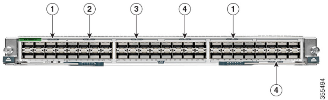
Figure 20: Example Interface Allocation for Port Groups on the Cisco Nexus 7000 Series 10-Gbps Ethernet Modules (N7K-F348XP-25)
