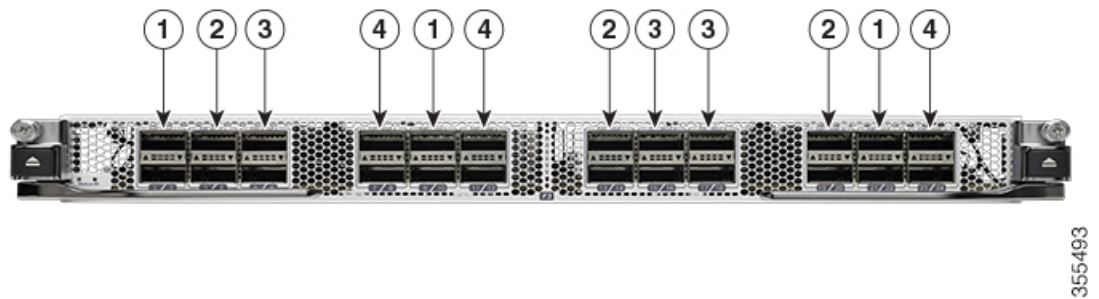
Figure 19: Example Interface Allocation for Port Groups on the Cisco Nexus 7700 Series 40-Gbps Ethernet Modules (N77-F324FQ-25)
