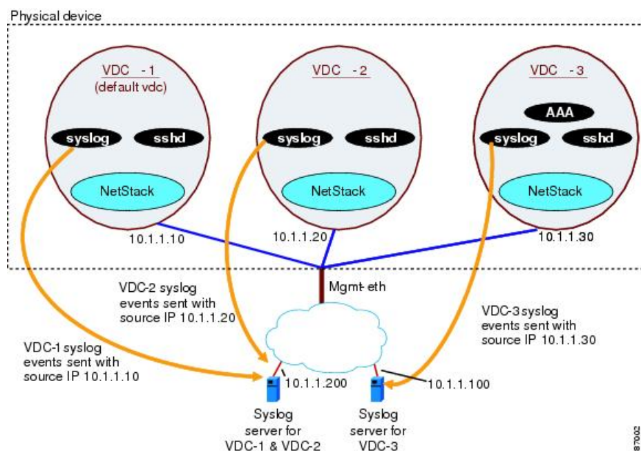
Figure 11: Out-of-Band VDC Management Example
