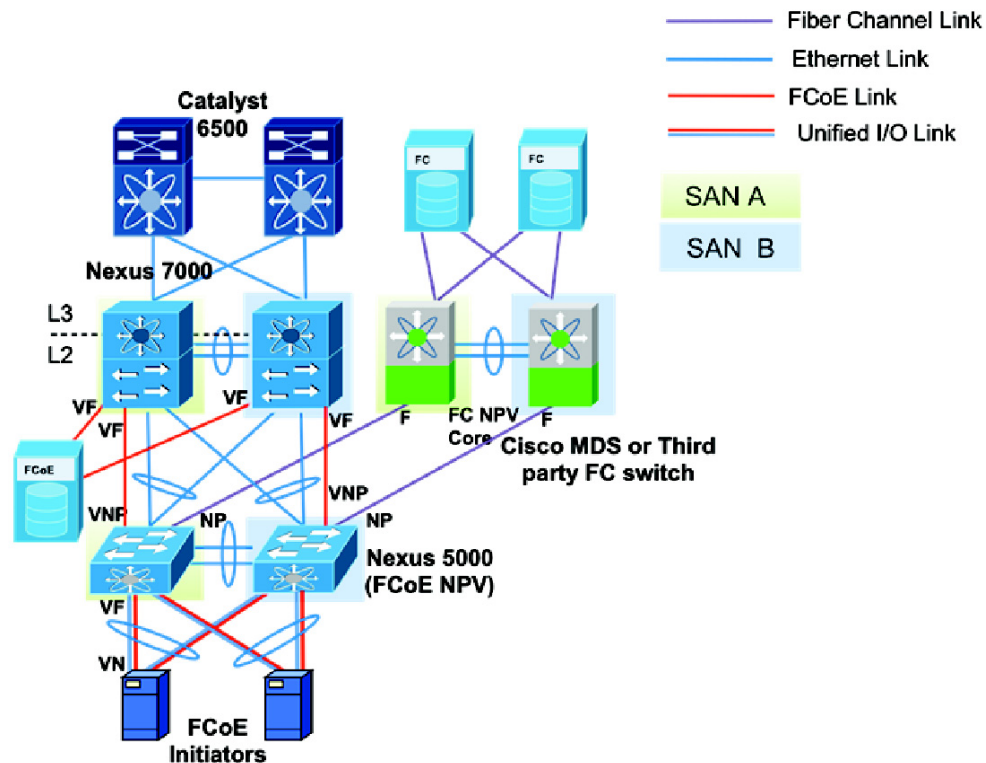
Figure 6-2 Converged Multi-hop FCoE Network Design Using FCoE NPV
