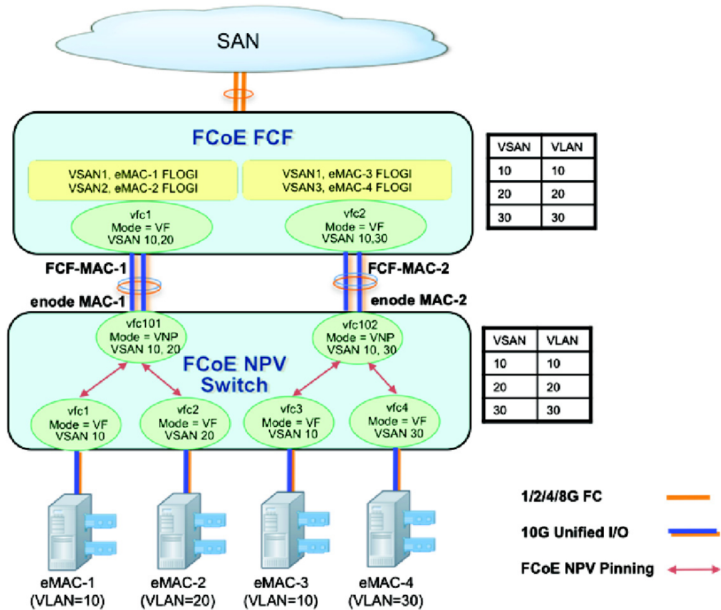
Figure 6-1 FCoE NPV Pinning, FLOGI-Based on VSANs
