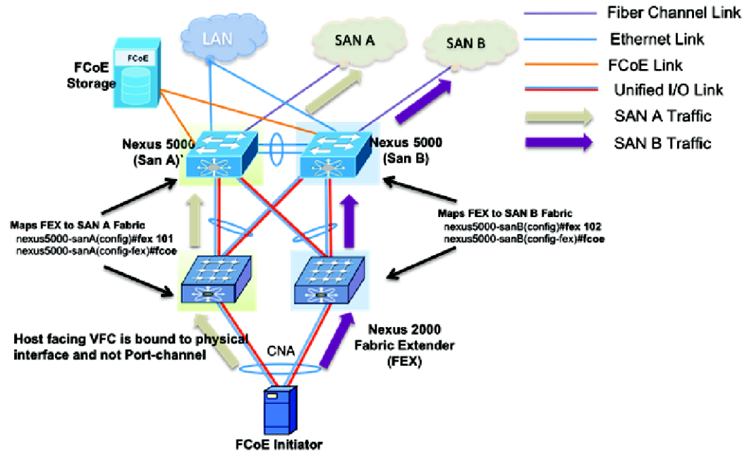
Figure 6-3 FCoE Network Design Using eVPC-layer vPC
