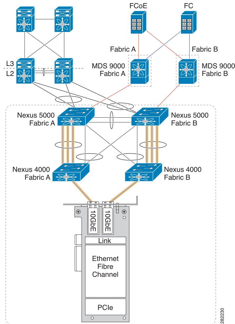
Figure 1-9 Cisco Nexus 4000 Series Switch Connected To A Cisco Nexus 5000 Series Switch FCoE With Dedicated Wires
