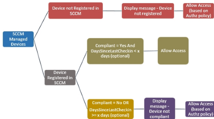
Figure 35: SCCM Workflow
