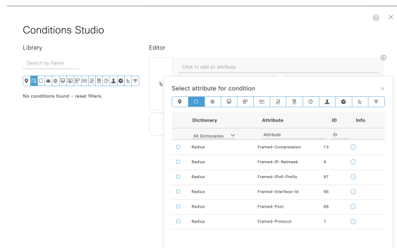
Figure 66: Conditions Studio
