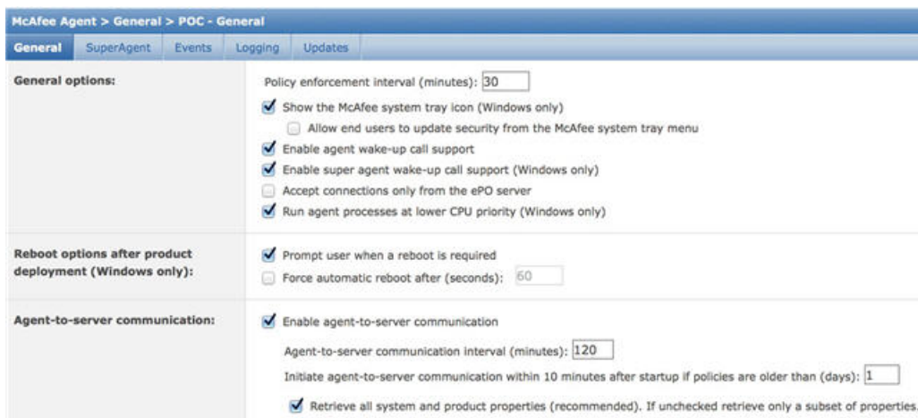
Figure 26: McAfee ePO Agent Recommended Options
