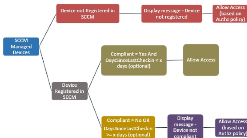
Figure 47: SCCM Workflow
