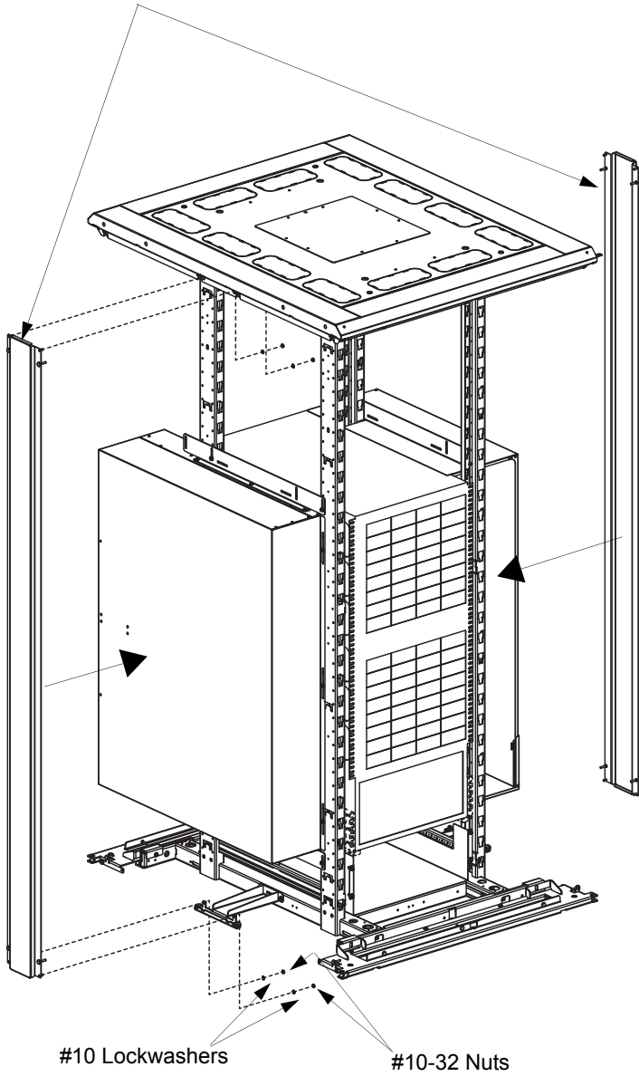
Vertical Side Supports
