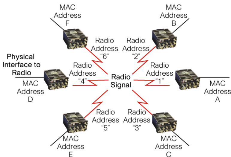
Figure 5. A Simple Radio Network
