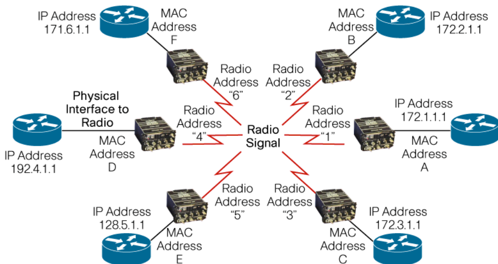
Figure 6. Radio Network with Internet Routers
