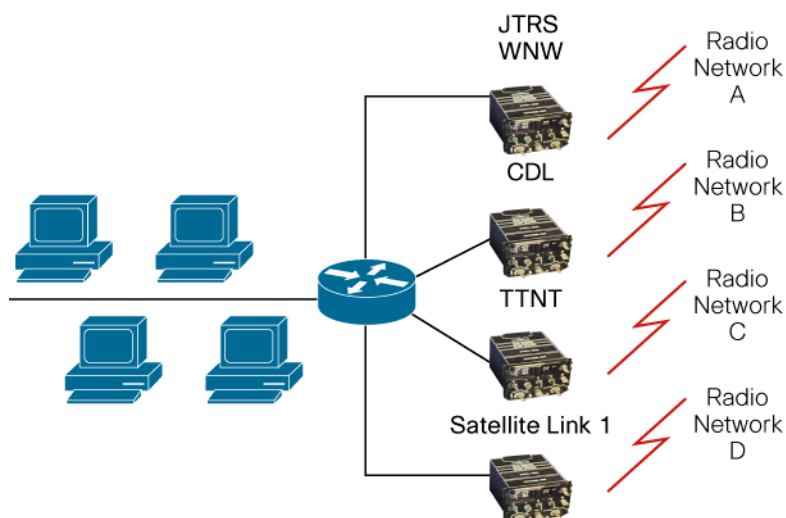
Figure 10. Standard Router to Radio Interfaces
