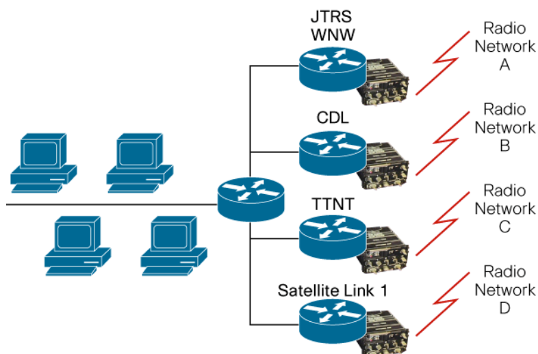
Figure 9. End Systems with Dedicated Aggregation Router
