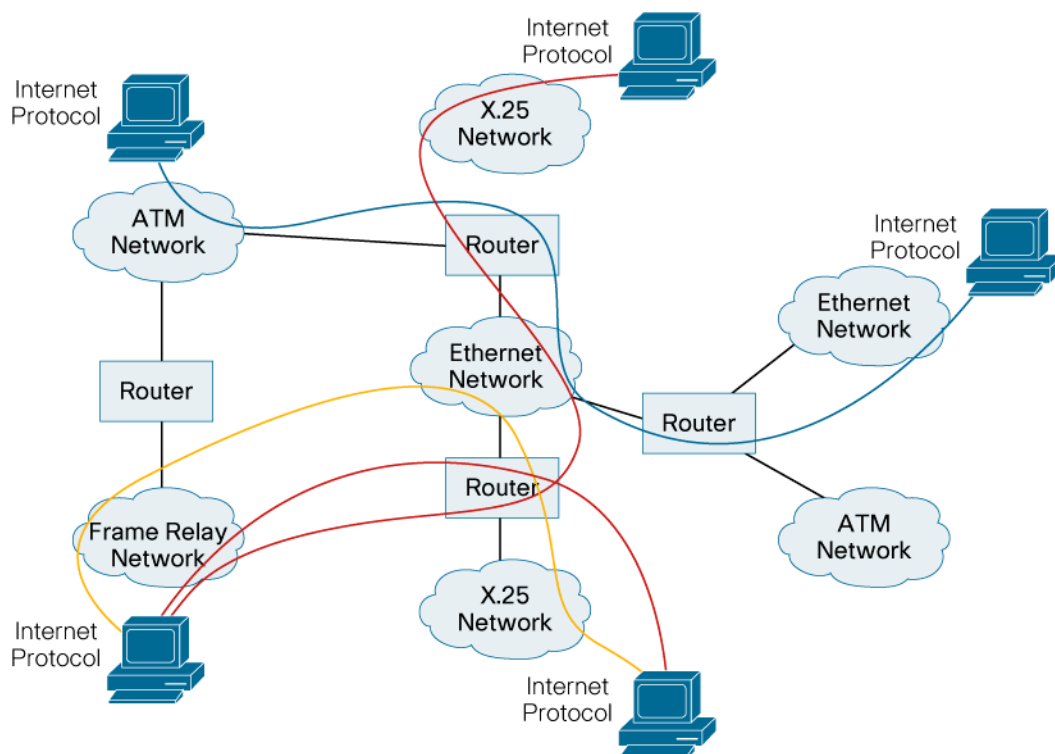
Figure 1. Internet Structure
