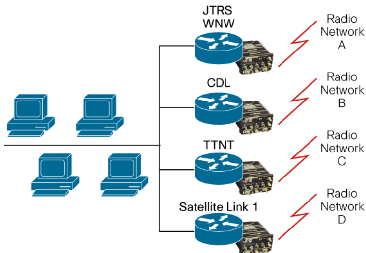
Figure 8. End Systems with Multiple Radio Types
