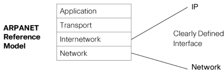
Figure 4. The ARPANET Reference Model
