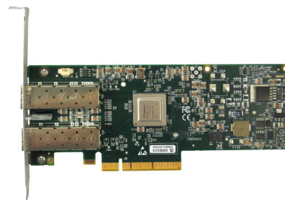
Figure 3: Mellanox ConnectX EN with RoE NICs (Dual SFP+ Card shown)
