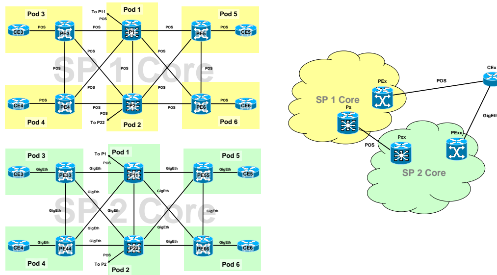
Figure 1. Lab Topology of Cisco IOS XR Advanced IPv4 Routing for Service Providers
