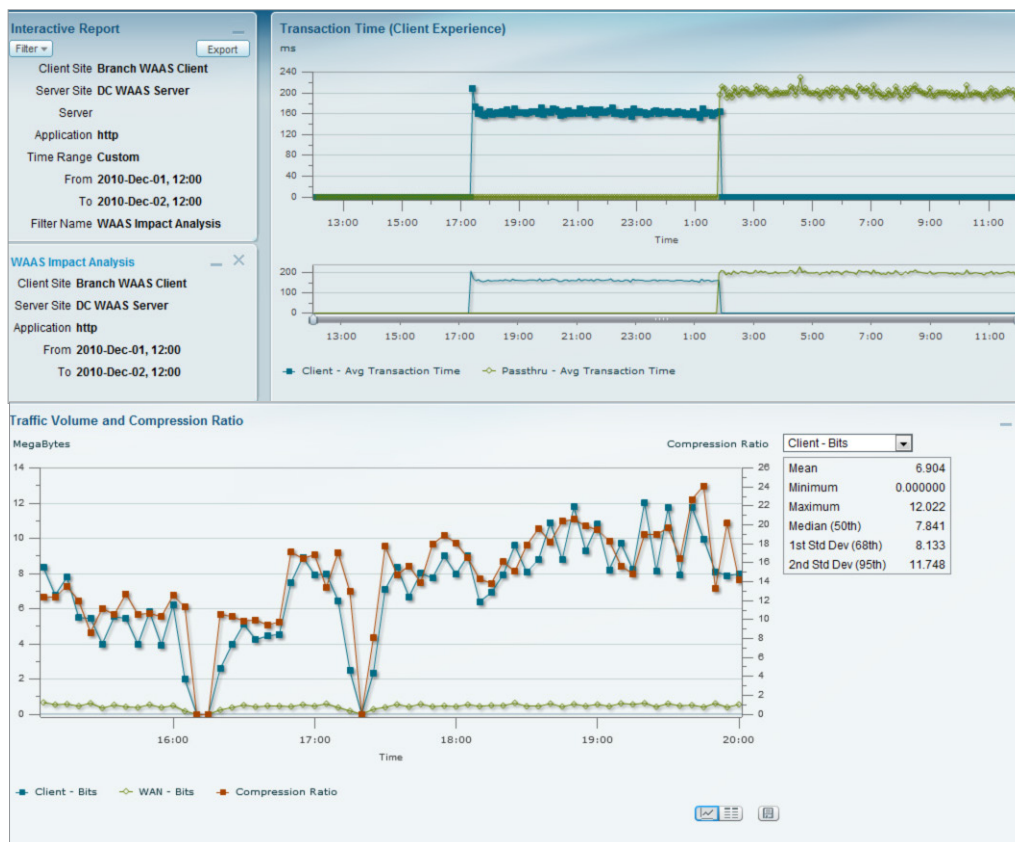
Figure 2. Historical views of WAN Optimization impact
