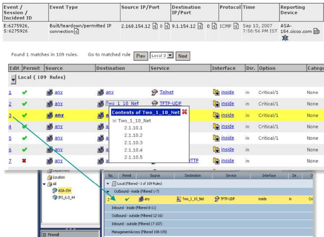
Figure 4. Cisco Security MARS Firewall Log to Cisco Security Manager Policy Collaboration
