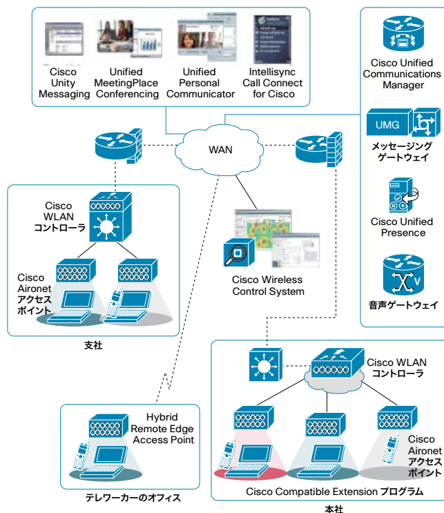
図 1 Cisco Unified Communications over WLAN
