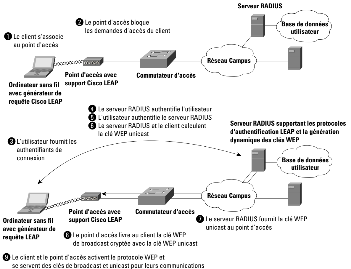
Figure 2 Processus d'authentification LEAP
