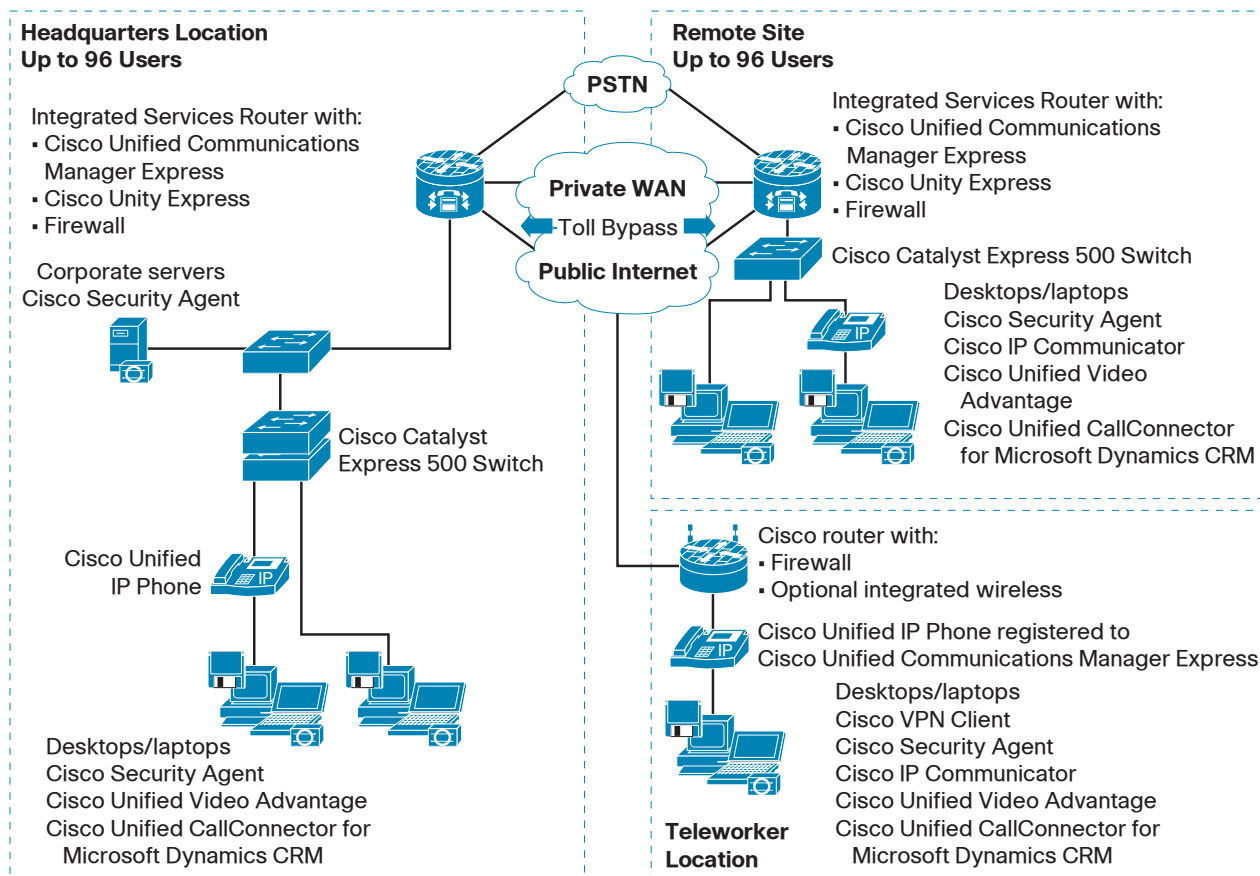
Figure 2. Cisco Unified Communications Solution Blueprint for Headquarters (up to 96 Users) with Multiple Branches (up to 96 Users) and Distributed Local Call Processing
