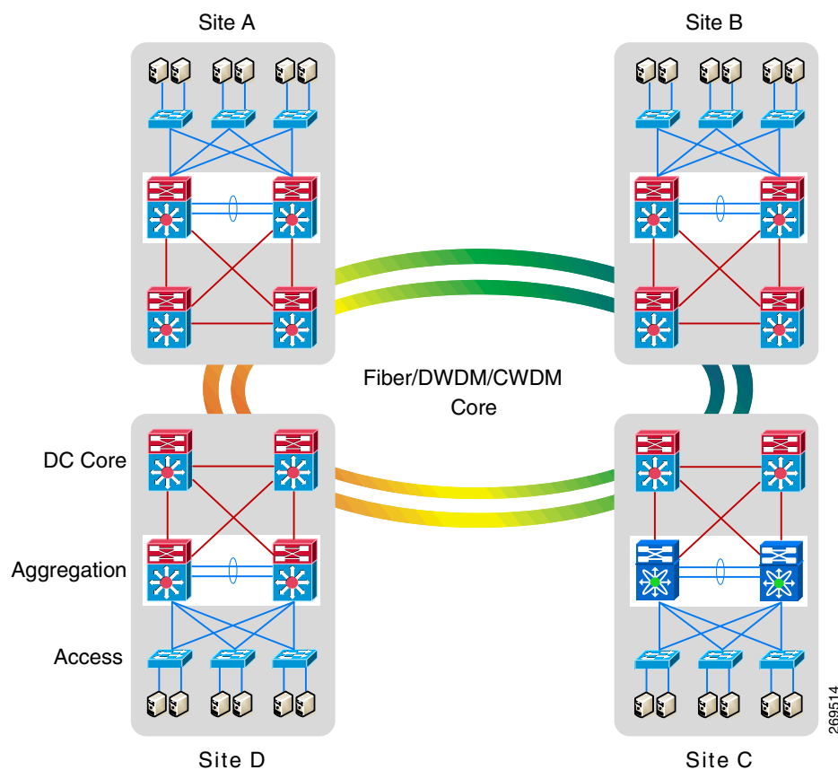
Figure 2-1 DCI Fiber, DWDM, and CWDM Core Topology
