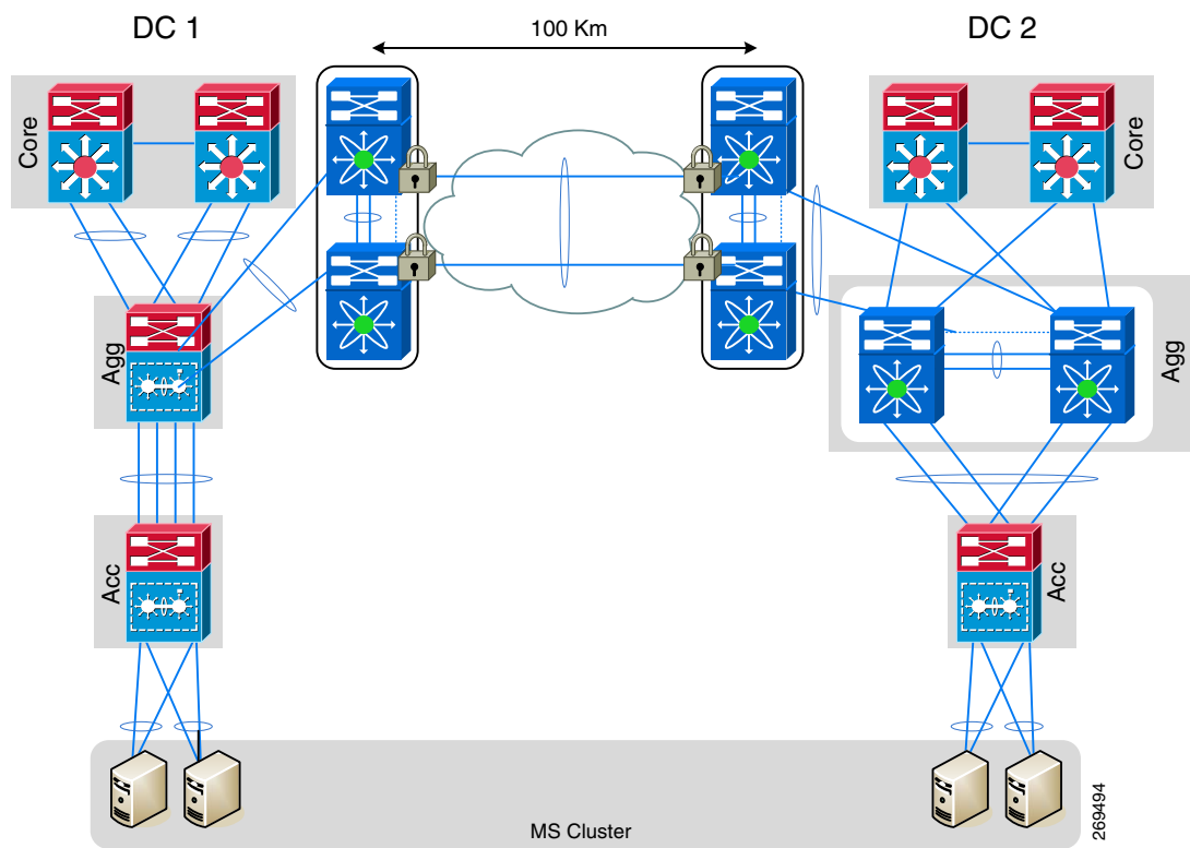
Figure 2-5 vPC-vPC (with 802.1AE) 2-Site Test Topology
