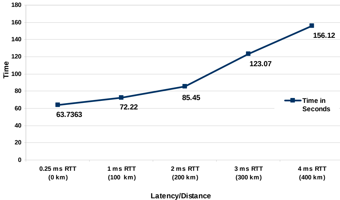
Figure 5. Duration of Intra- and Inter-Data Center VMware VMotion Migration
