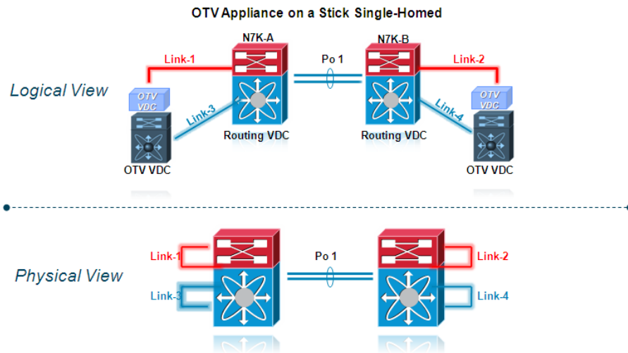
Figure 1-28 Single-homed OTV VDC
