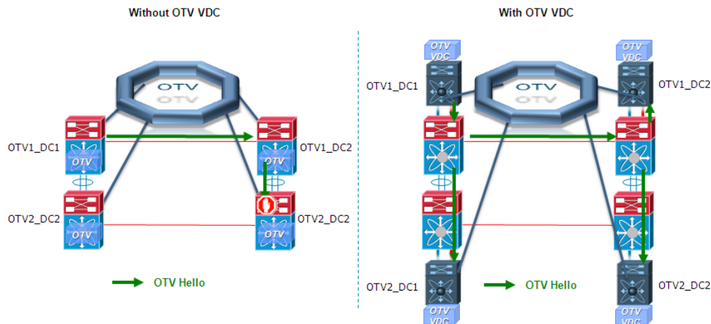
Figure 1-41 Delivery of OTV Hello Packets on Join Interface
