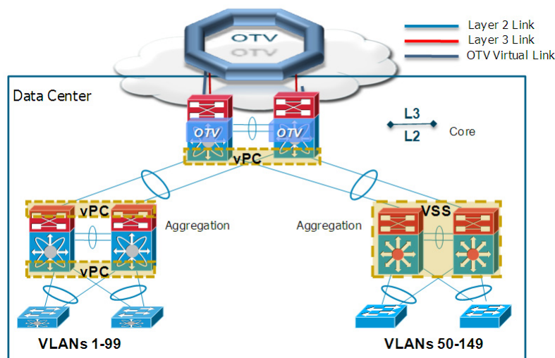
Figure 1-36 OTV in the Core (Layer 2-Layer 3 Boundary at the Core)
