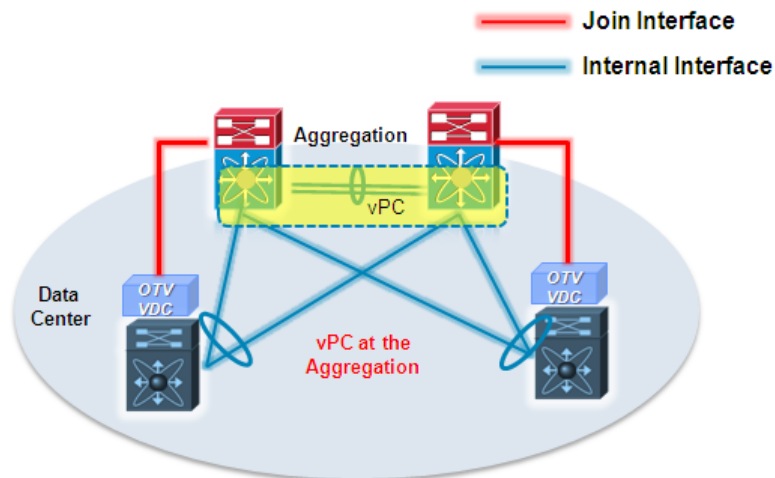
Figure 1-46 vPC Based Design
