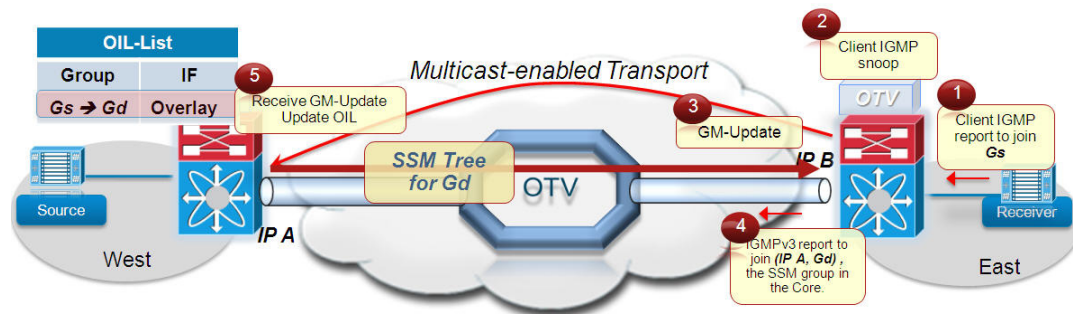
Figure 1-11 Receiver Joining the Multicast Group Gs
