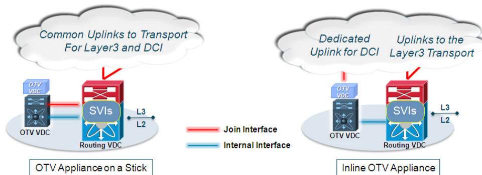
Figure 1-27 OTV VDC Models
