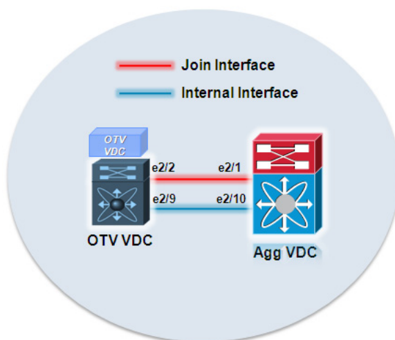
Figure 1-48 OTV Configuration Topology of Reference
