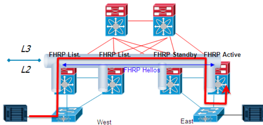
Figure 1-25 Suboptimal Outbound Routing
