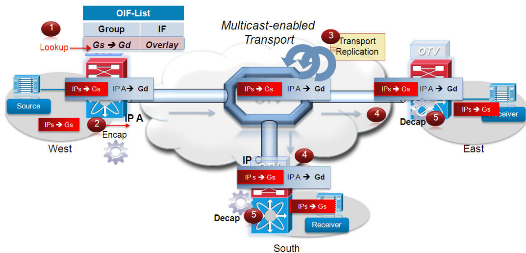
Figure 1-12 Delivery of the Multicast Stream Gs
