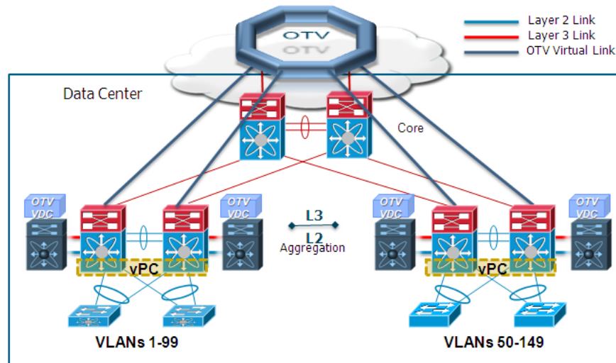
Figure 1-38 OTV at the Aggregation Layer
