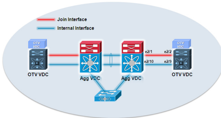
Figure 1-49 OTV Multi-Homing Configuration
