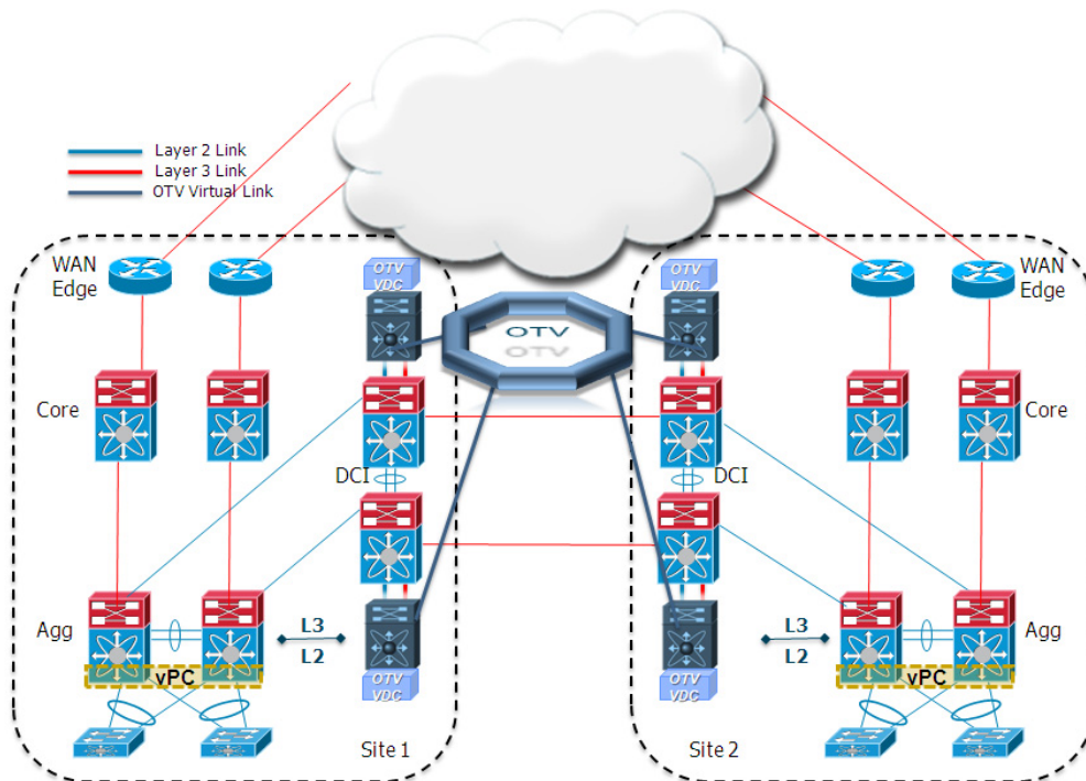
Figure 1-40 Point-to-Point OTV Deployments with Dedicated DCI Layer
