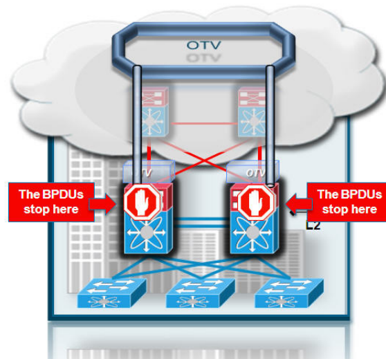
Figure 1-13 OTV Spanning Tree Isolation
