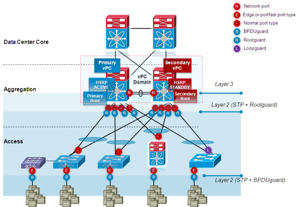
Figure 1-43 STP Data Center Best Practices
