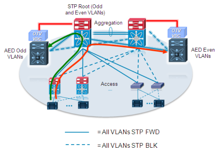
Figure 1-44 Single STP Root for All the VLANs
