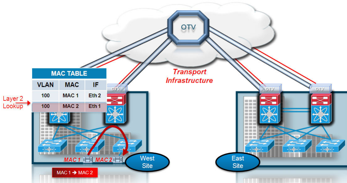
Figure 1-7 Intra Site Layer 2 Unicast Traffic
