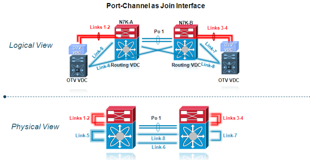
Figure 1-30 Use of Port Channel as Join Interface
