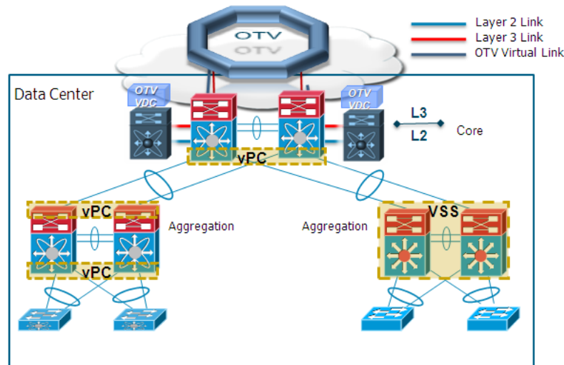
Figure 1-37 OTV VDCs at the Core Layer
