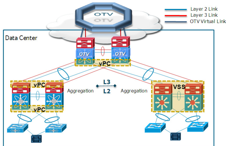
Figure 1-32 OTV in the Core (Layer 2-Layer 3 Boundary at the Aggregation)
