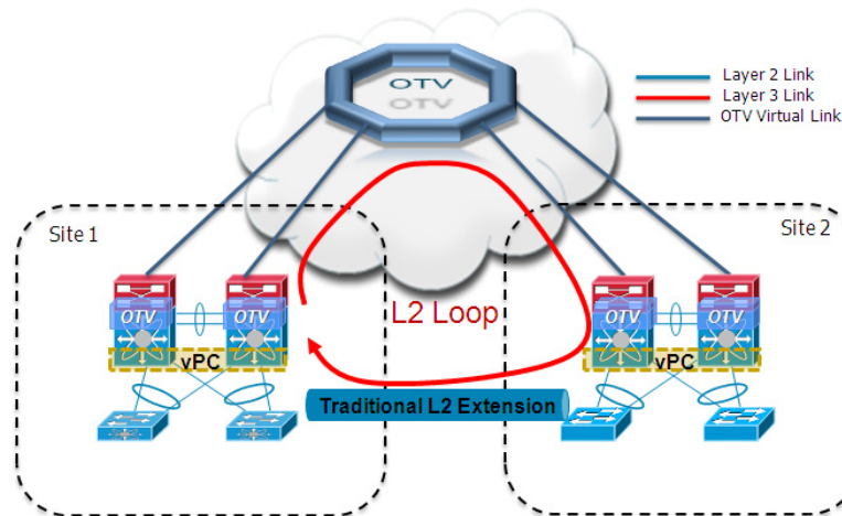
Figure 1-20 Creation of an End-to-End Loop
