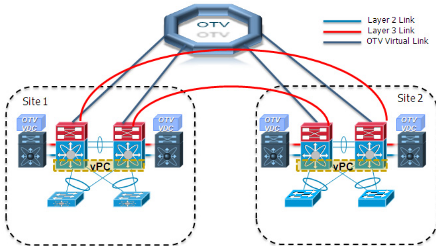
Figure 1-39 Point-to-Point OTV Deployments with Collapsed DC Aggregation/Core
