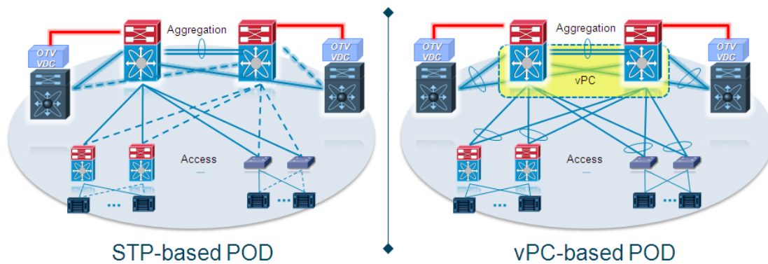
Figure 1-42 OTV VDC Site Transparency
