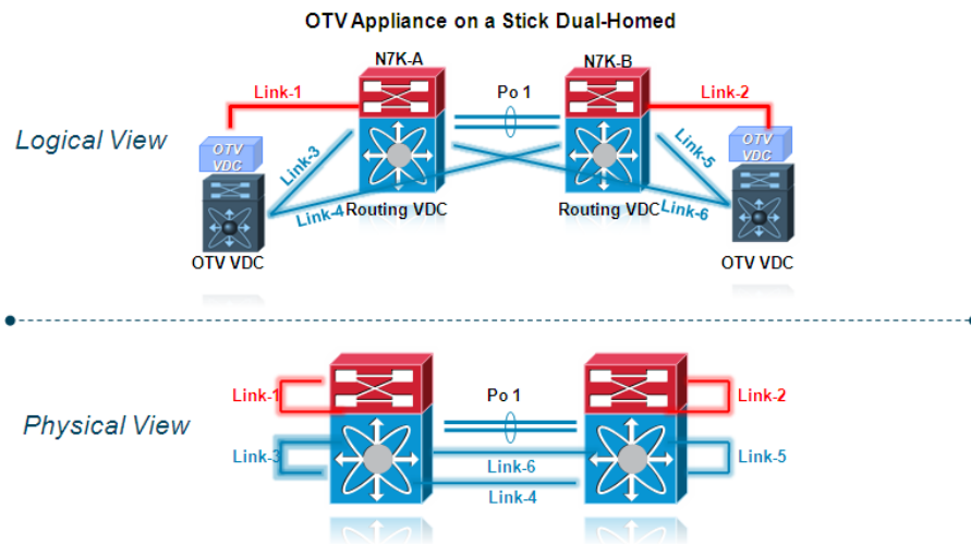
Figure 1-29 OTV Appliance on a Stick
