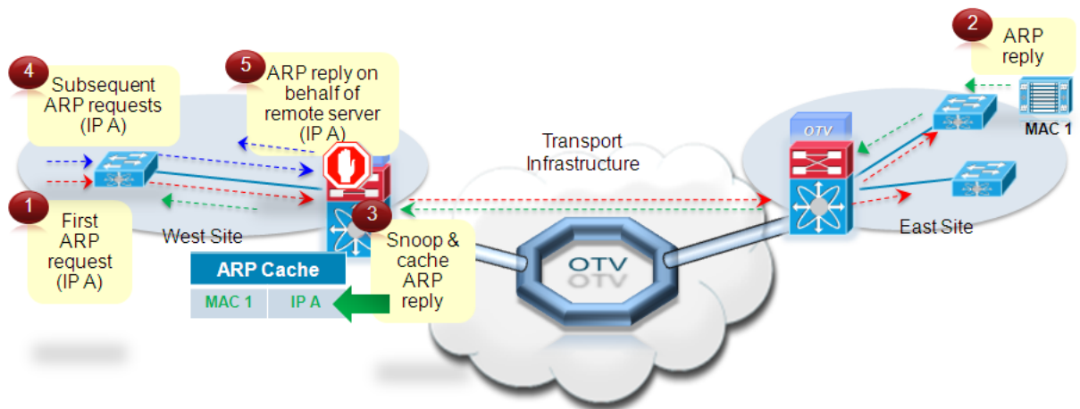
Figure 1-15 OTV ARP Optimization
