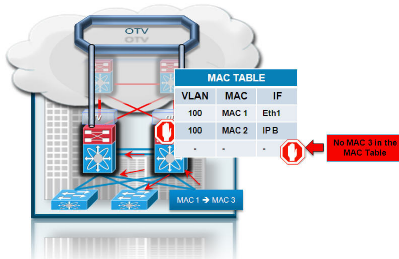
Figure 1-14 OTV Unknown Unicast Handling
