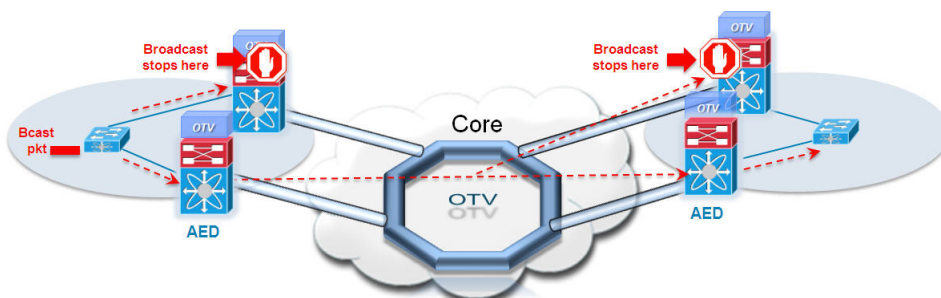
Figure 1-19 Prevention of End-to-End STP Loops
