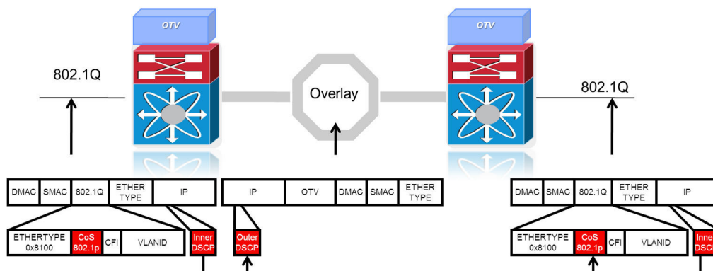
Figure 1-24 Default QoS Behavior of the OTV Edge Device
