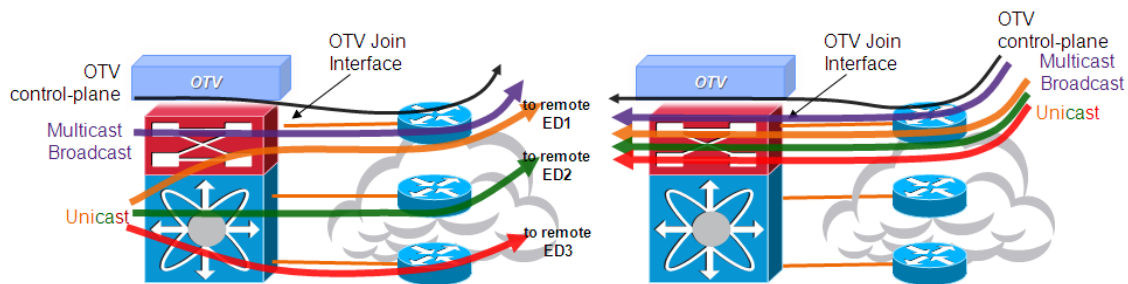
Figure 1-22 Inbound and Outbound Traffic Paths
