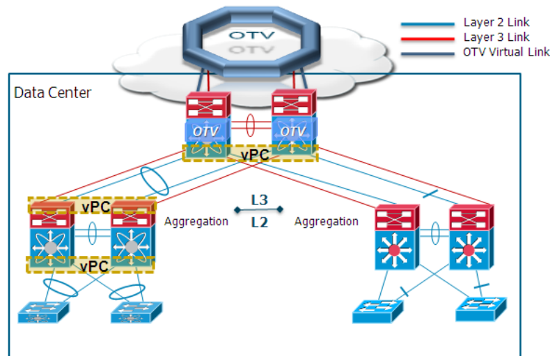
Figure 1-34 OTV in the Core with non MCEC Capable POD Devices
