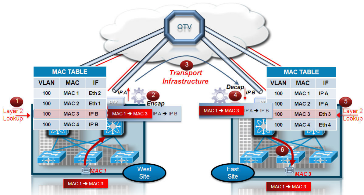
Figure 1-8 Inter Site Layer 2 Unicast Traffic
