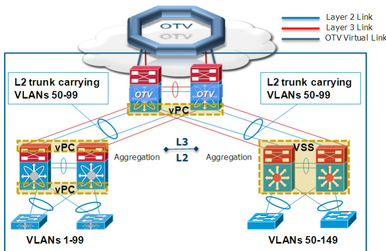
Figure 1-33 Layer 2 Connectivity Intra- and Inter- Data Center
