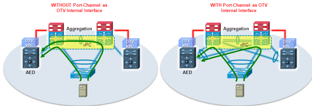
Figure 1-47 Traffic Flow Considerations
