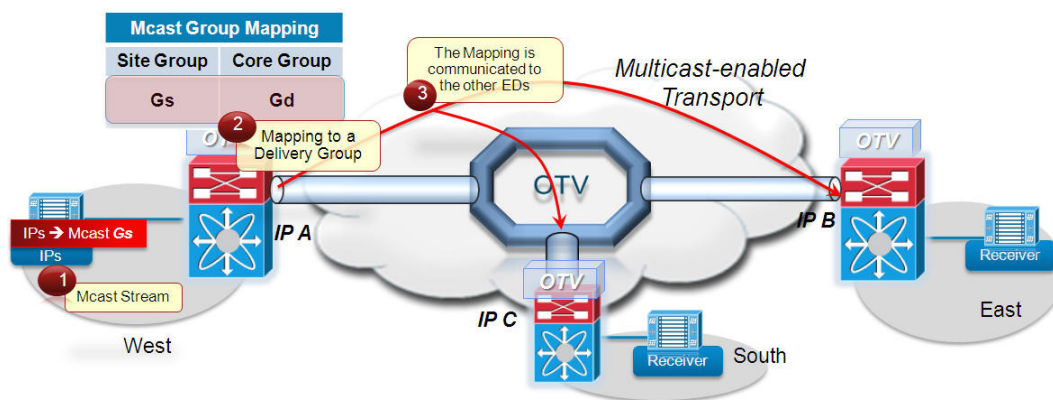
Figure 1-10 Multicast Source Streaming to Group Gs
