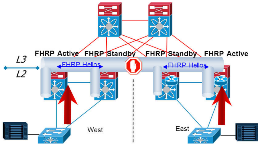
Figure 1-26 FHRP Isolation with OTV
