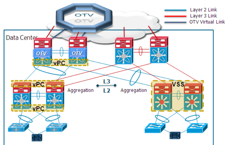
Figure 1-35 OTV Deployed on Dedicated Devices
