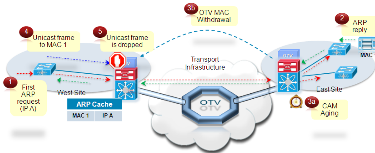
Figure 1-16 Traffic Black-Holing Scenario
