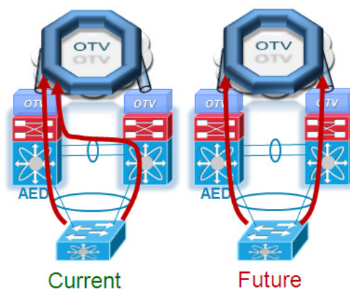
Figure 1-21 Unicast Traffic Load Balancing
