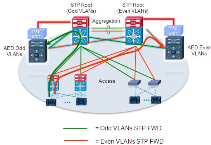
Figure 1-45 Different STP Root for Odd and Even VLANs
