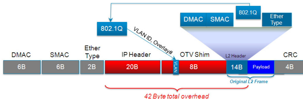
Figure 1-9 OTV Data Plane Encapsulation
