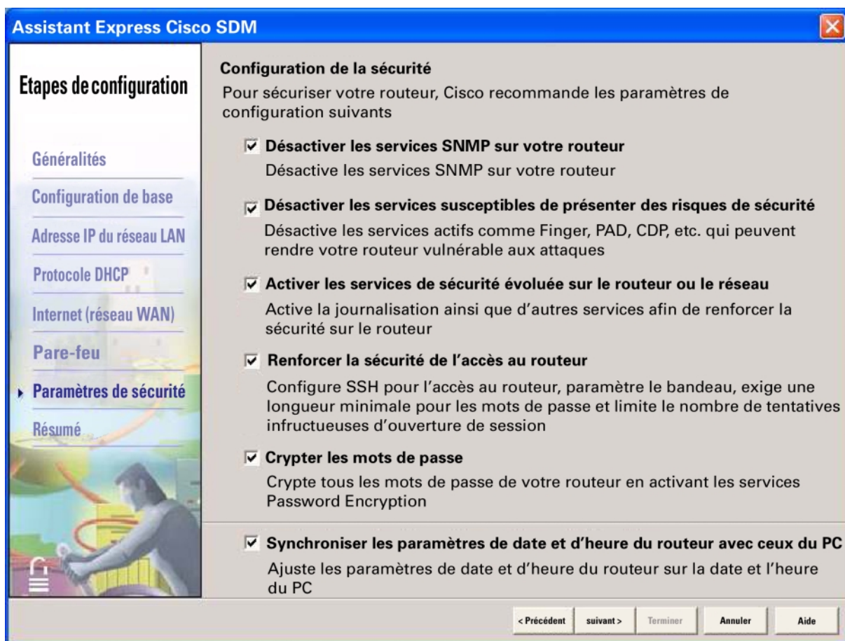
Figure 3. Cisco SDM
