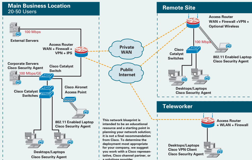
Figure 1: Network Blueprint for Small and Medium-Sized Businesses with 20 to 50 User Ports per Site
