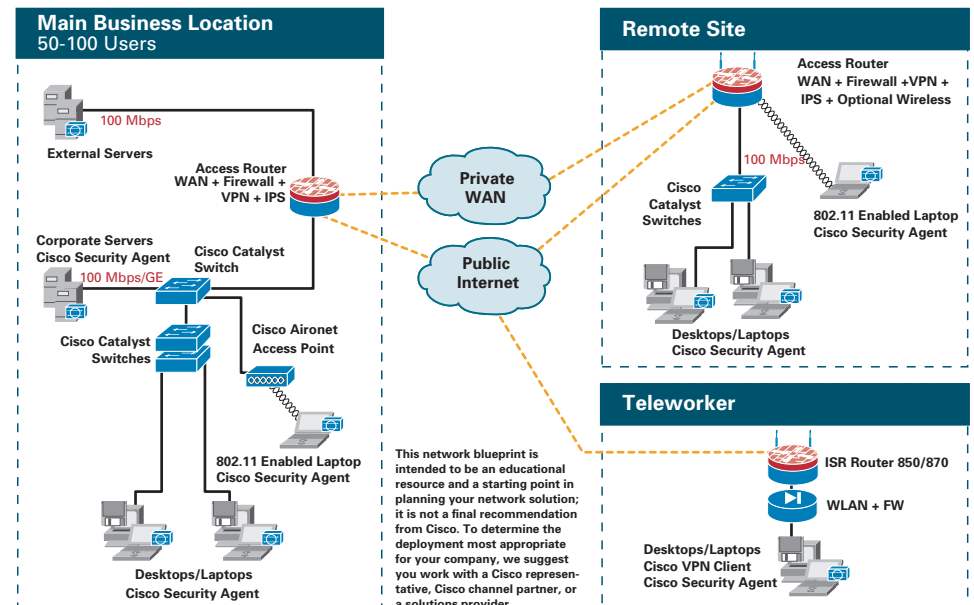
Figure 2: Network Blueprint for Small and Medium-Sized Businesses with 50 to 100 User Ports per Site
