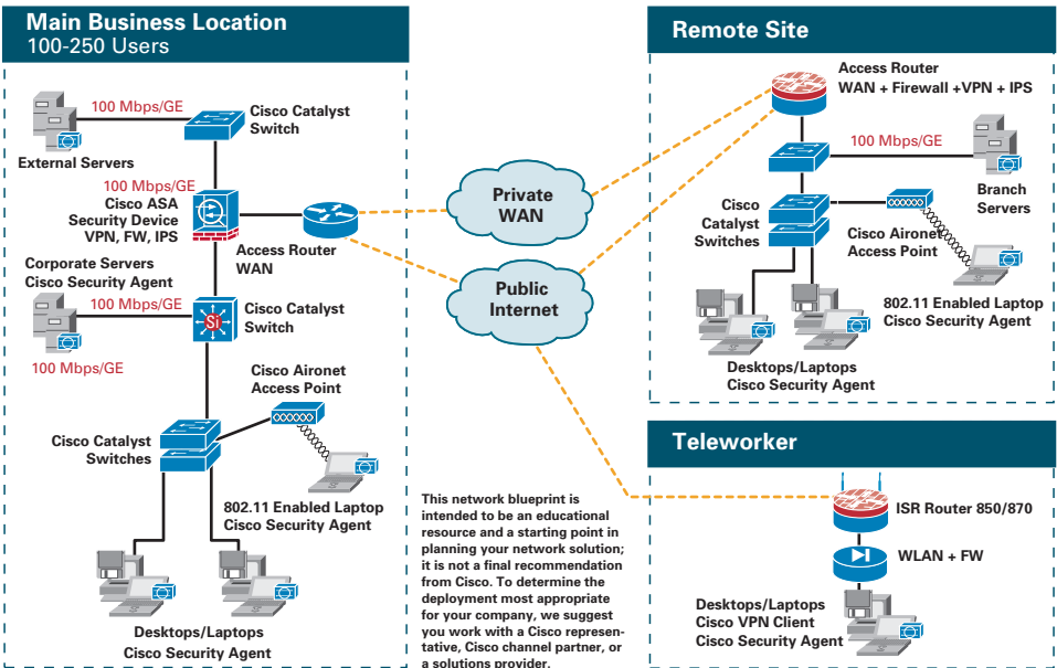
Figure 3: Network Blueprint for Small and Medium-Sized Businesses with 100 to 250 User Ports per Site
