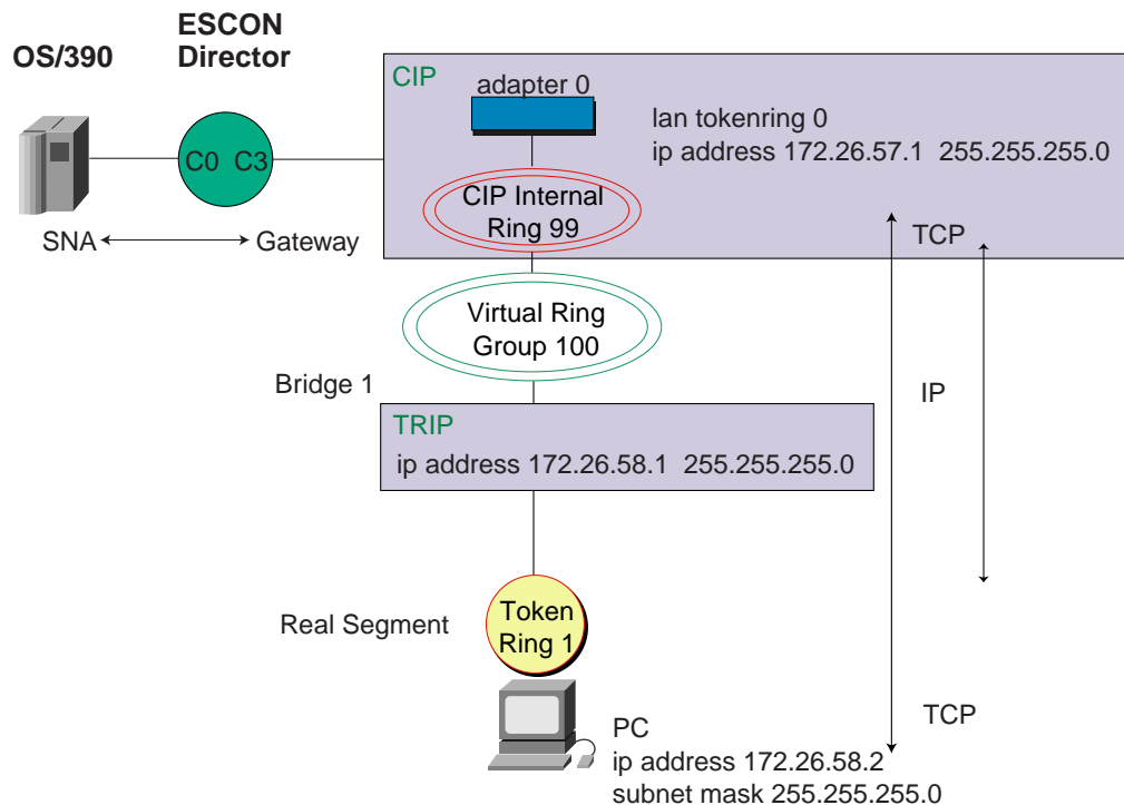
Figure 1 TN3270 Server Network Scenario
