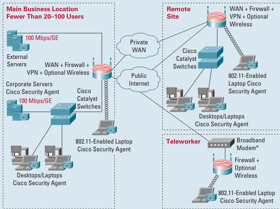
Figure 1: Network Diagram for SMBs with 20–100 User Ports per Site
