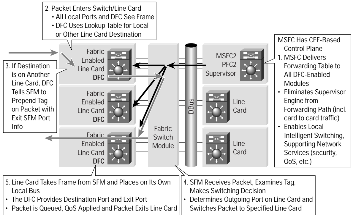
Figure 5 Distributed Cisco Express Forwarding Packet Flow
