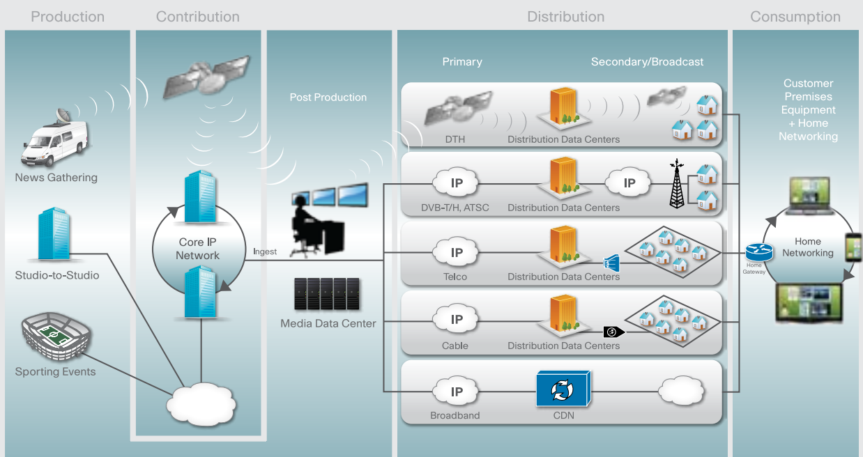
Figure 1: Medianet Architecture
