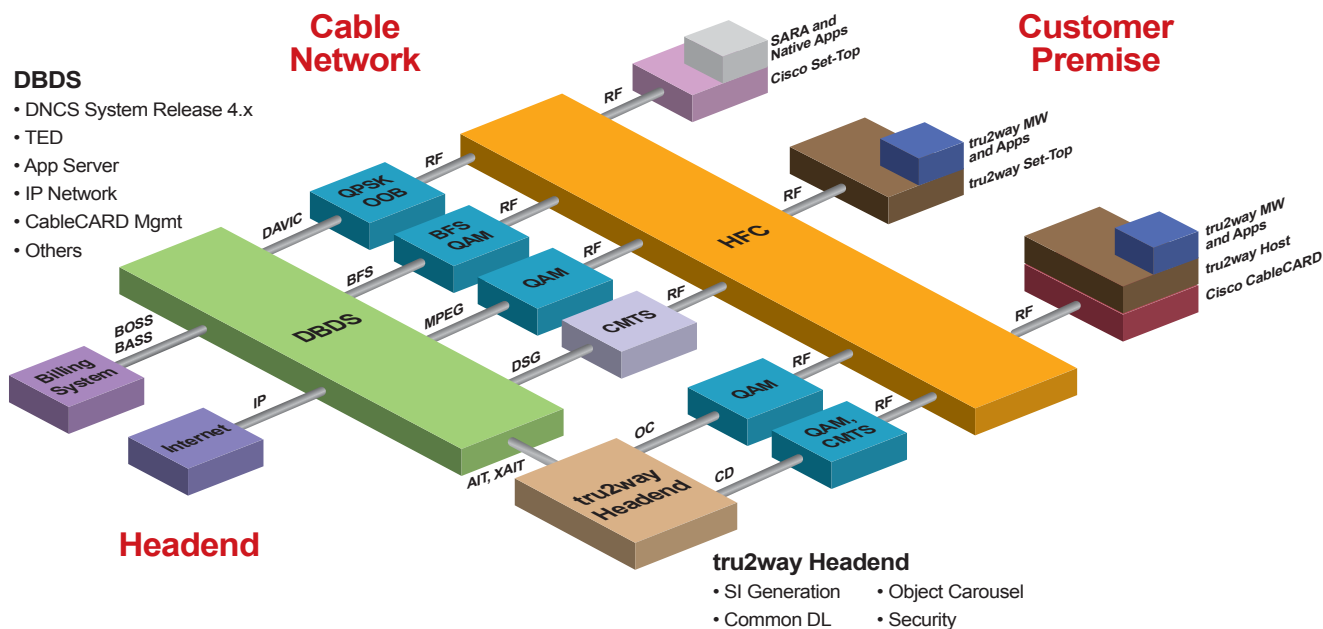
Cisco's tru2way Solution Works Within the Existing Cable Network and Plant
