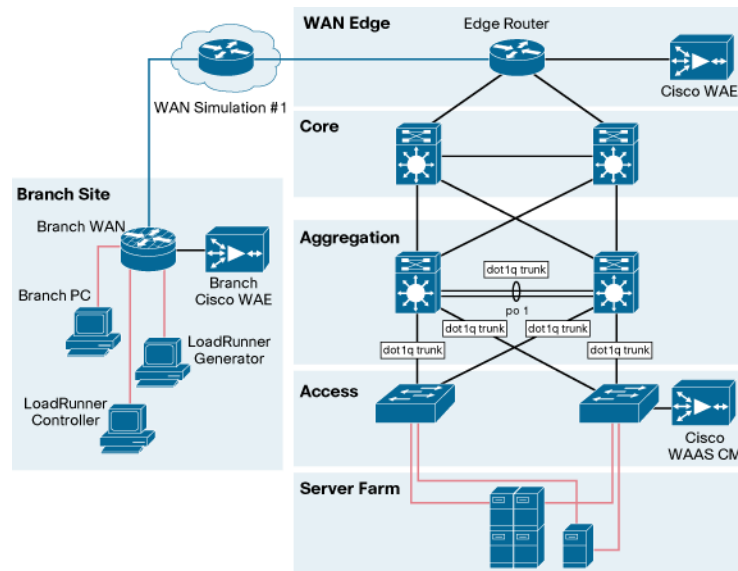
Figure 3. Cisco Application Networking Architecture for BEA WebLogic
