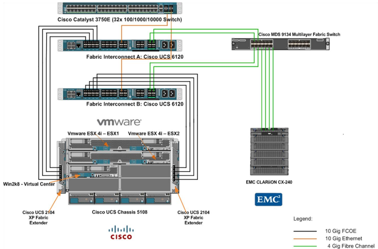
Figure 3. Physical Architecture
