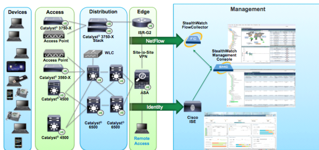
Figure 1 Cyber Threat Defense Solution 1.1. Architecture
