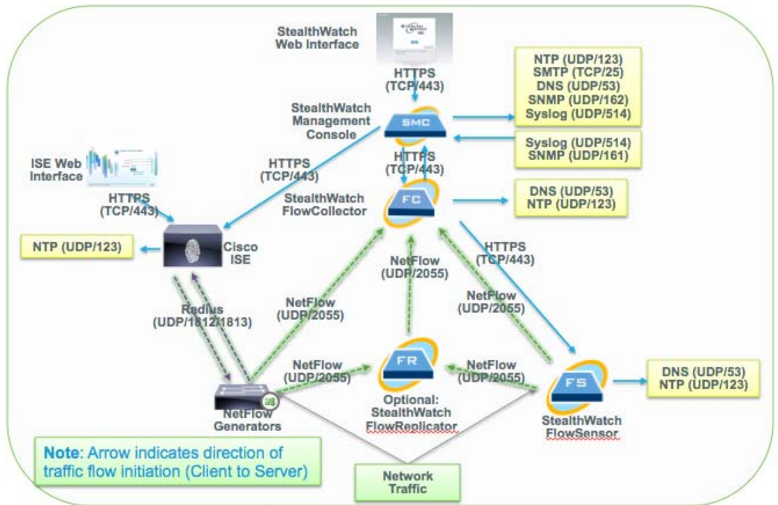
Figure 3 Cisco Cyber Threat Defense Solution 1.1 Data Flows
