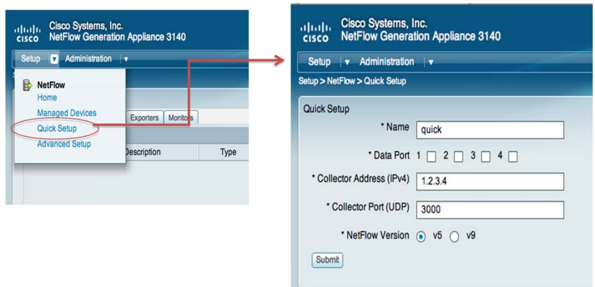
Figure 10 Quick Setup
