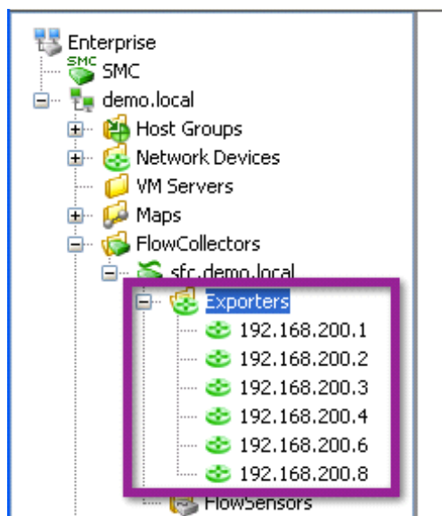
Figure 12 Expanded Tree
