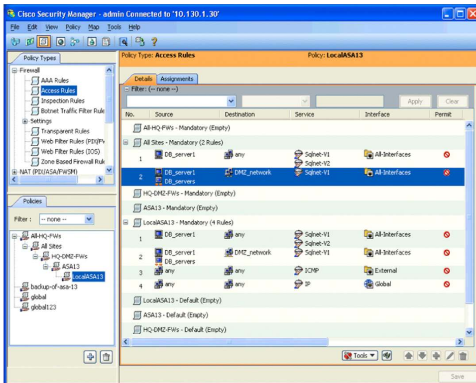
Figure 1. Security Policy Management
