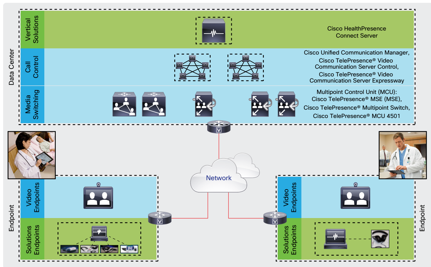
Figure 1. Cisco HealthPresence Deployment
