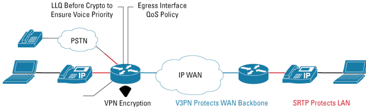
Figure 5. Secure, Toll Quality IP Telephony with SRTM
